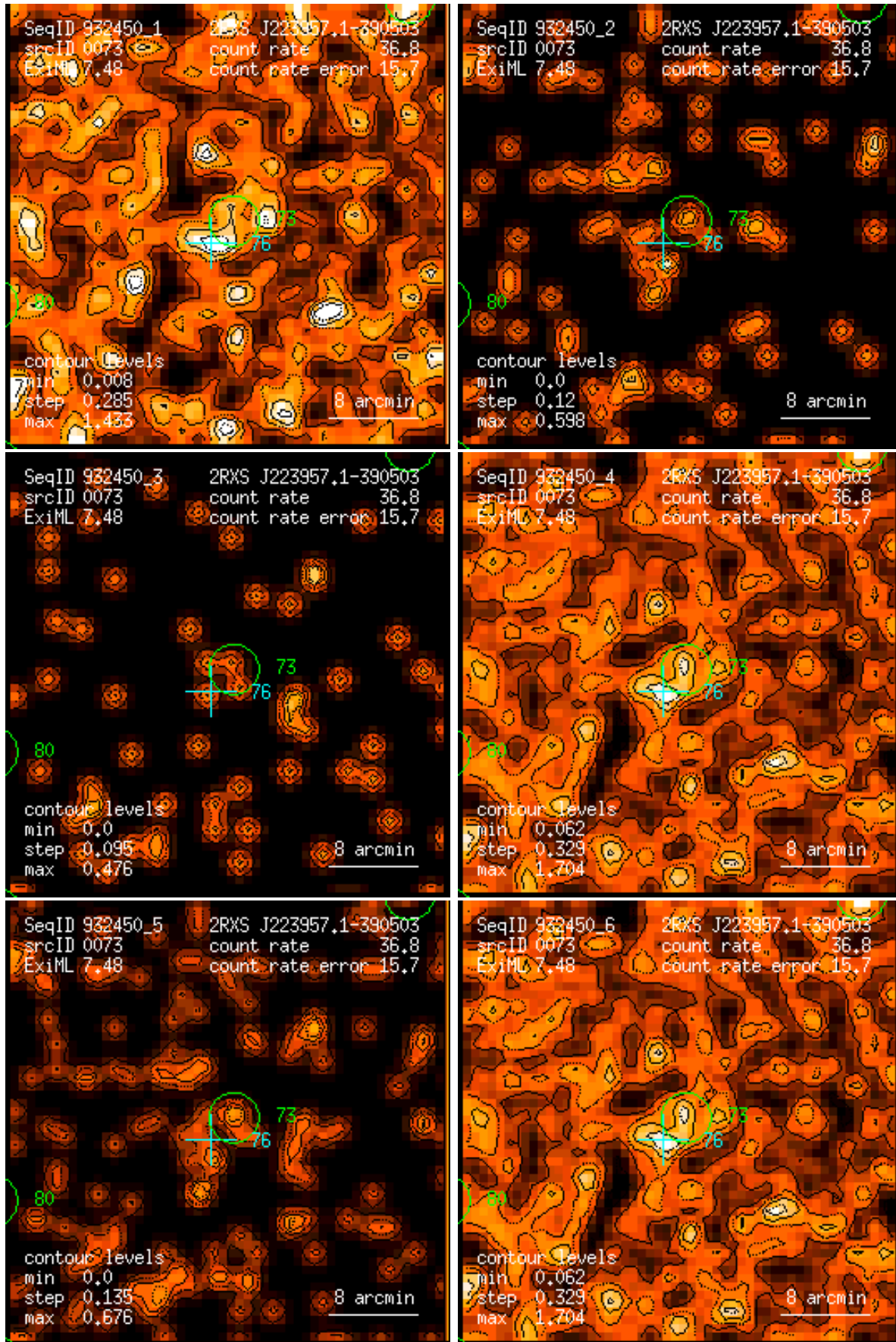
Figure 73: RASS 932450: detection 0073: band rate images, Gaussian filter: (1) PSPC channels 11 – 41, (2) 52 – 90, (3) 91 – 201, (4) 11 – 235, (5) 52 – 201, (6) 11 – 201. Broad band rates in counts/ks. Band rate contour levels in counts/ks/arcmin 2 .
