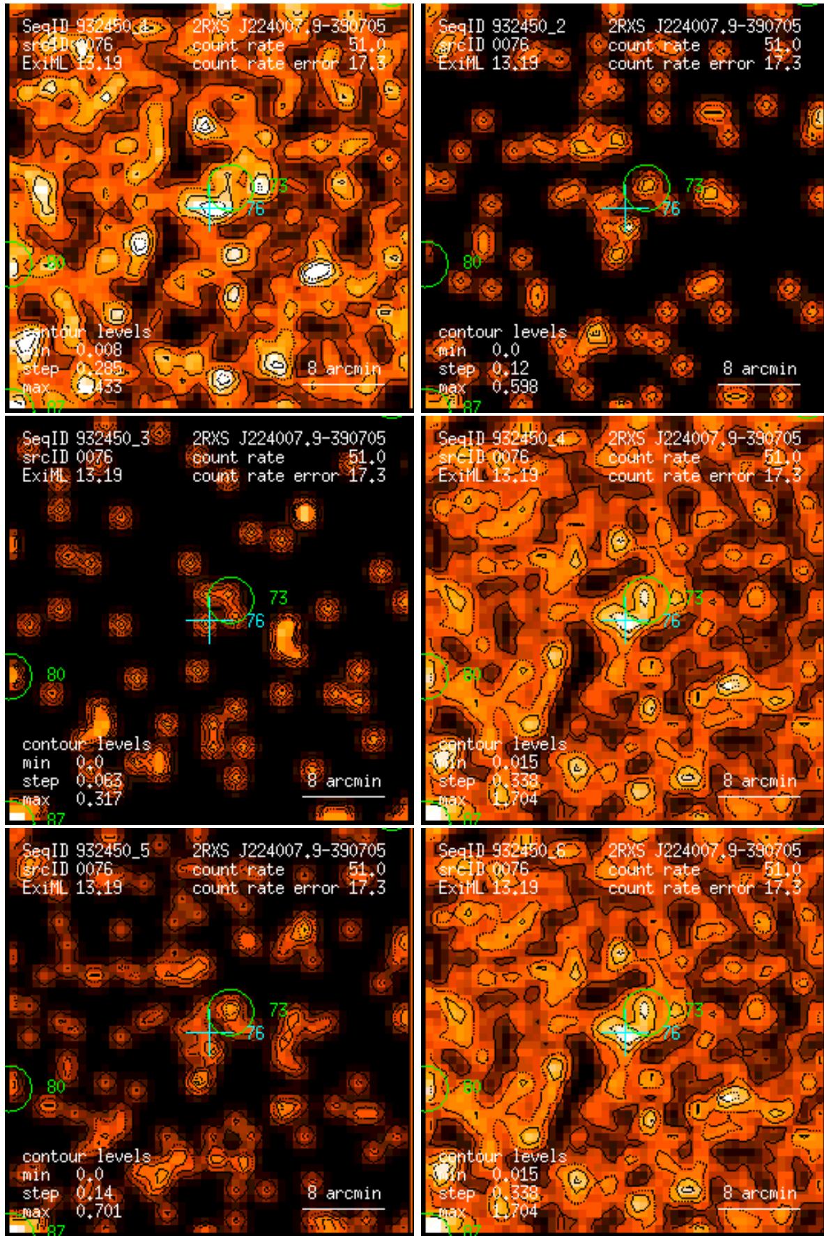
Figure 76: RASS 932450: detection 0076: band rate images, Gaussian filter: (1) PSPC channels 11 – 41, (2) 52 – 90, (3) 91 – 201, (4) 11 – 235, (5) 52 – 201, (6) 11 – 201. Broad band rates in counts/ks. Band rate contour levels in counts/ks/arcmin 2 .
