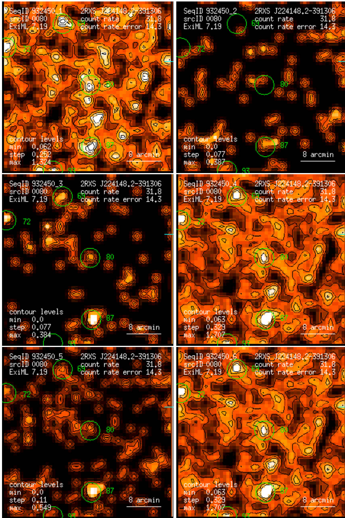
Figure 80: RASS 932450: detection 0080: band rate images, Gaussian filter: (1) PSPC channels 11 – 41, (2) 52 – 90, (3) 91 – 201, (4) 11 – 235, (5) 52 – 201, (6) 11 – 201. Broad band rates in counts/ks. Band rate contour levels in counts/ks/arcmin 2 .
