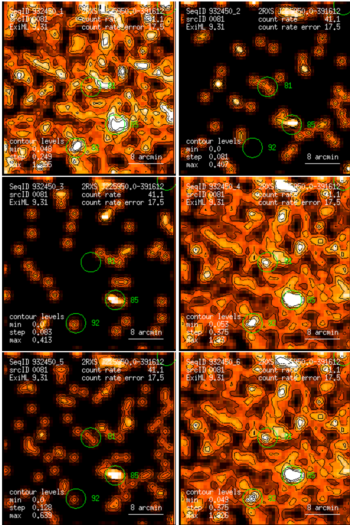
Figure 81: RASS 932450: detection 0081: band rate images, Gaussian filter: (1) PSPC channels 11 – 41, (2) 52 – 90, (3) 91 – 201, (4) 11 – 235, (5) 52 – 201, (6) 11 – 201. Broad band rates in counts/ks. Band rate contour levels in counts/ks/arcmin 2 .
