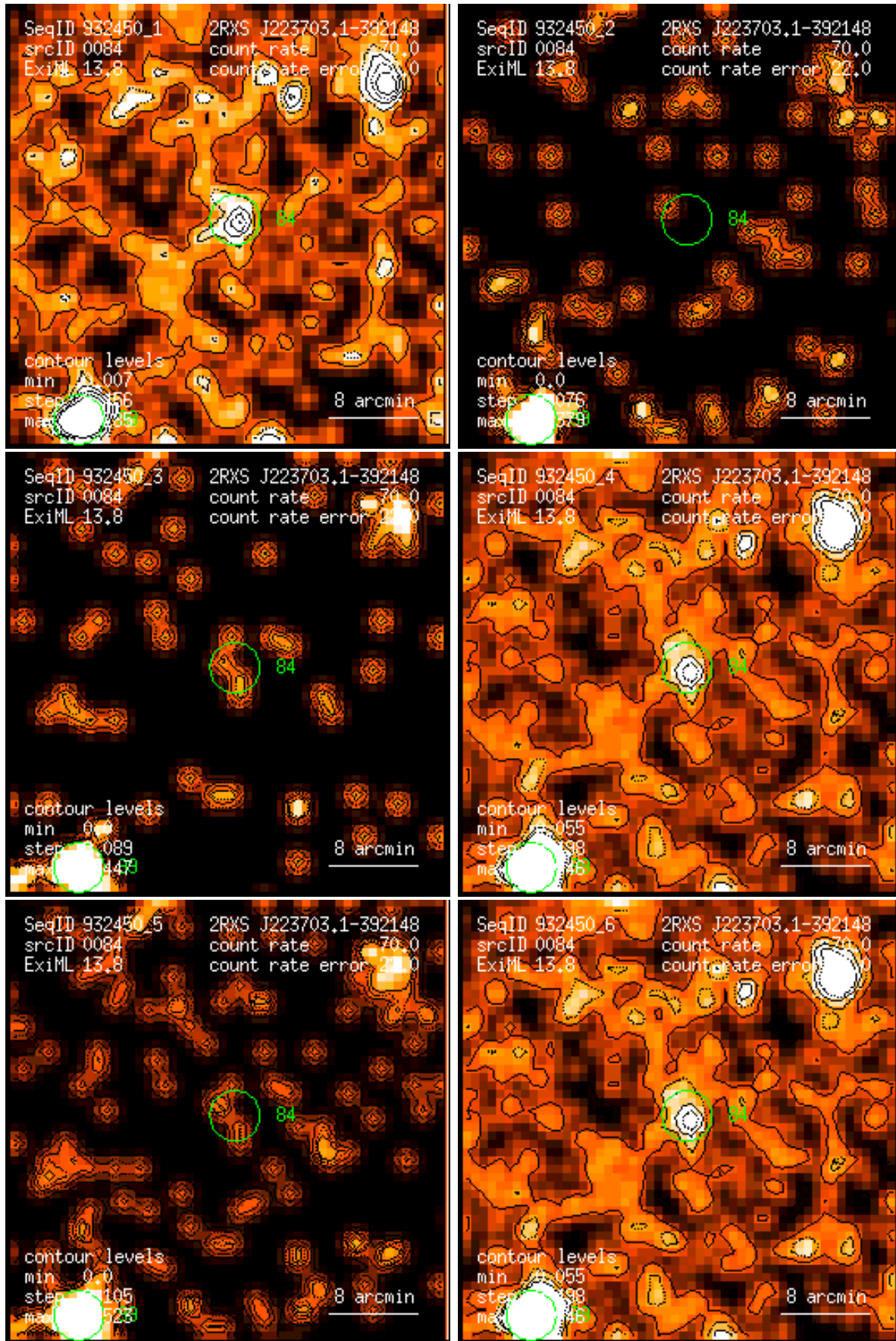
Figure 84: RASS 932450: detection 0084: band rate images, Gaussian filter: (1) PSPC channels 11 – 41, (2) 52 – 90, (3) 91 – 201, (4) 11 – 235, (5) 52 – 201, (6) 11 – 201. Broad band rates in counts/ks. Band rate contour levels in counts/ks/arcmin 2 .
