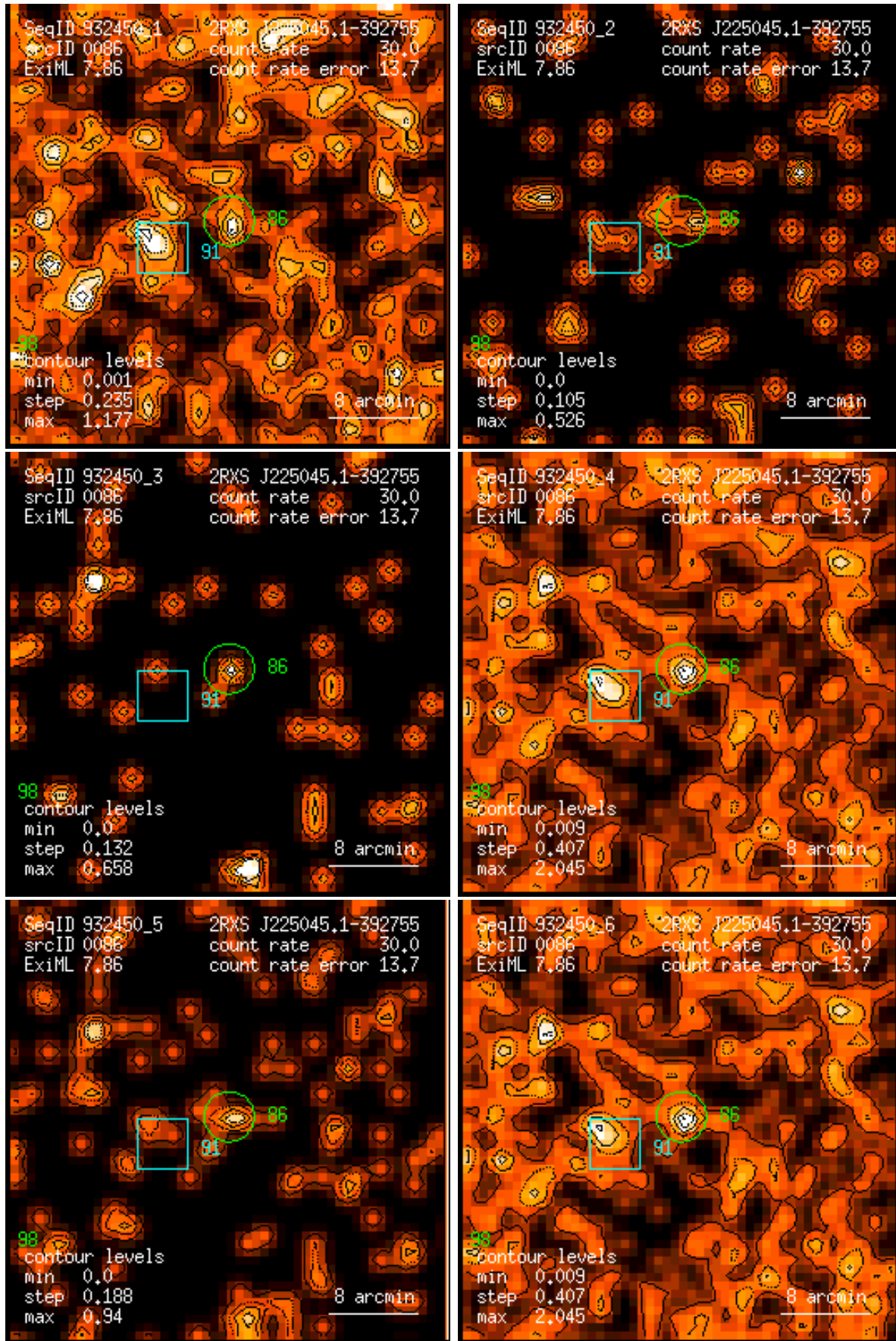
Figure 86: RASS 932450: detection 0086: band rate images, Gaussian filter: (1) PSPC channels 11 – 41, (2) 52 – 90, (3) 91 – 201, (4) 11 – 235, (5) 52 – 201, (6) 11 – 201. Broad band rates in counts/ks. Band rate contour levels in counts/ks/arcmin 2 .
