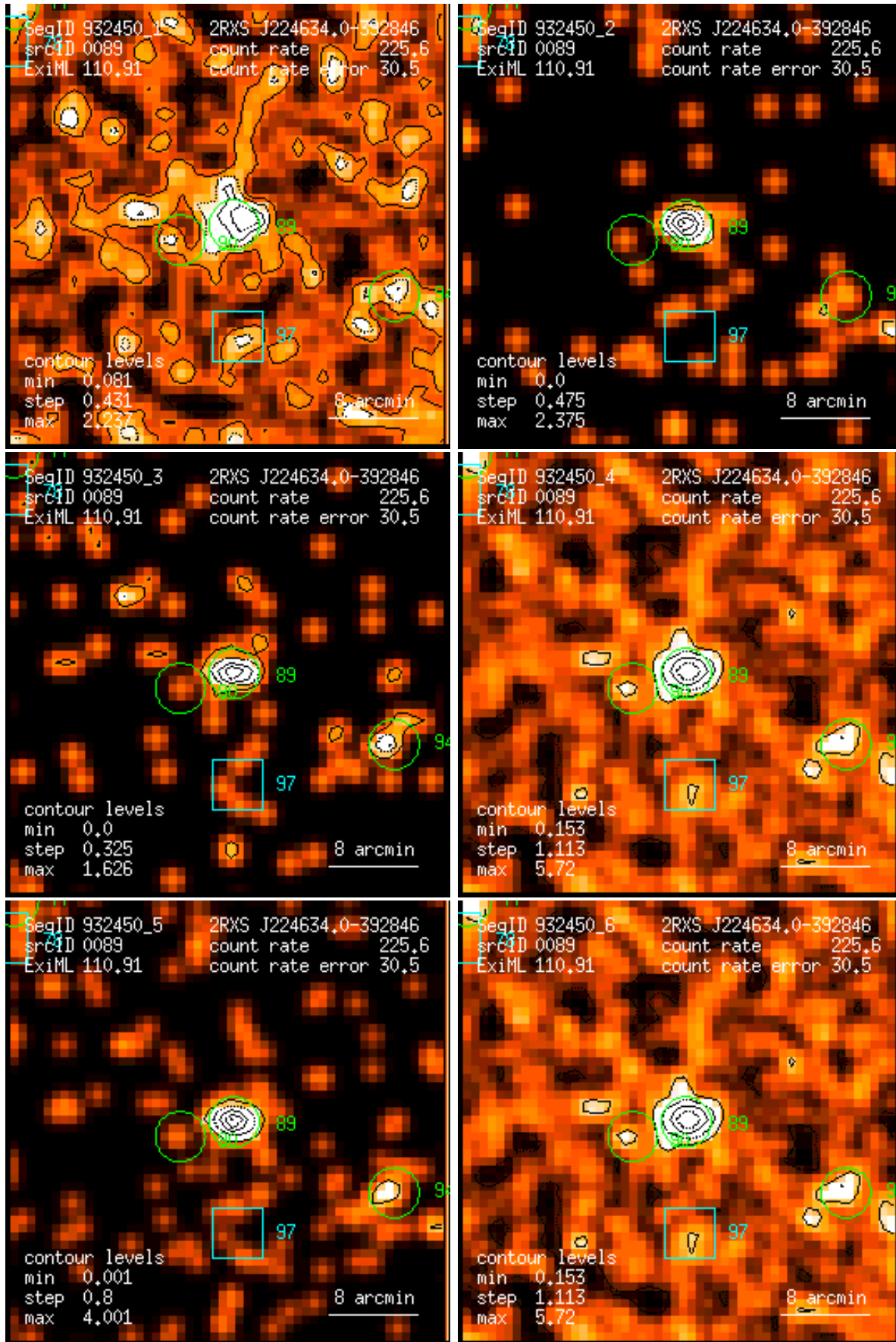
Figure 89: RASS 932450: detection 0089: band rate images, Gaussian filter: (1) PSPC channels 11 – 41, (2) 52 – 90, (3) 91 – 201, (4) 11 – 235, (5) 52 – 201, (6) 11 – 201. Broad band rates in counts/ks. Band rate contour levels in counts/ks/arcmin 2 .
