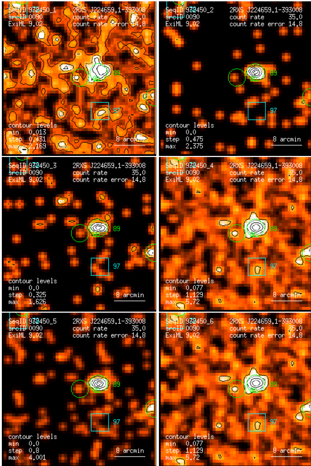
Figure 90: RASS 932450: detection 0090: band rate images, Gaussian filter: (1) PSPC channels 11 – 41, (2) 52 – 90, (3) 91 – 201, (4) 11 – 235, (5) 52 – 201, (6) 11 – 201. Broad band rates in counts/ks. Band rate contour levels in counts/ks/arcmin 2 .
