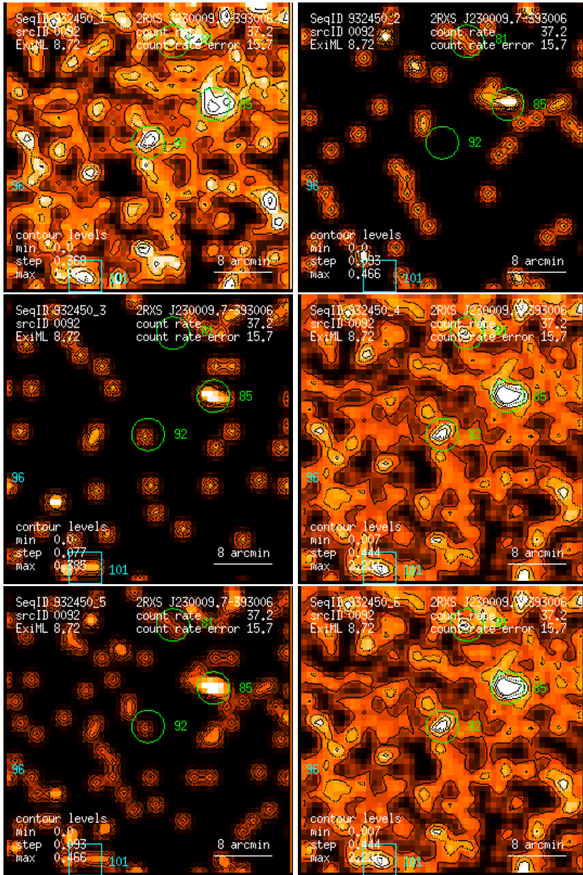
Figure 92: RASS 932450: detection 0092: band rate images, Gaussian filter: (1) PSPC channels 11 – 41, (2) 52 – 90, (3) 91 – 201, (4) 11 – 235, (5) 52 – 201, (6) 11 – 201. Broad band rates in counts/ks. Band rate contour levels in counts/ks/arcmin 2 .
