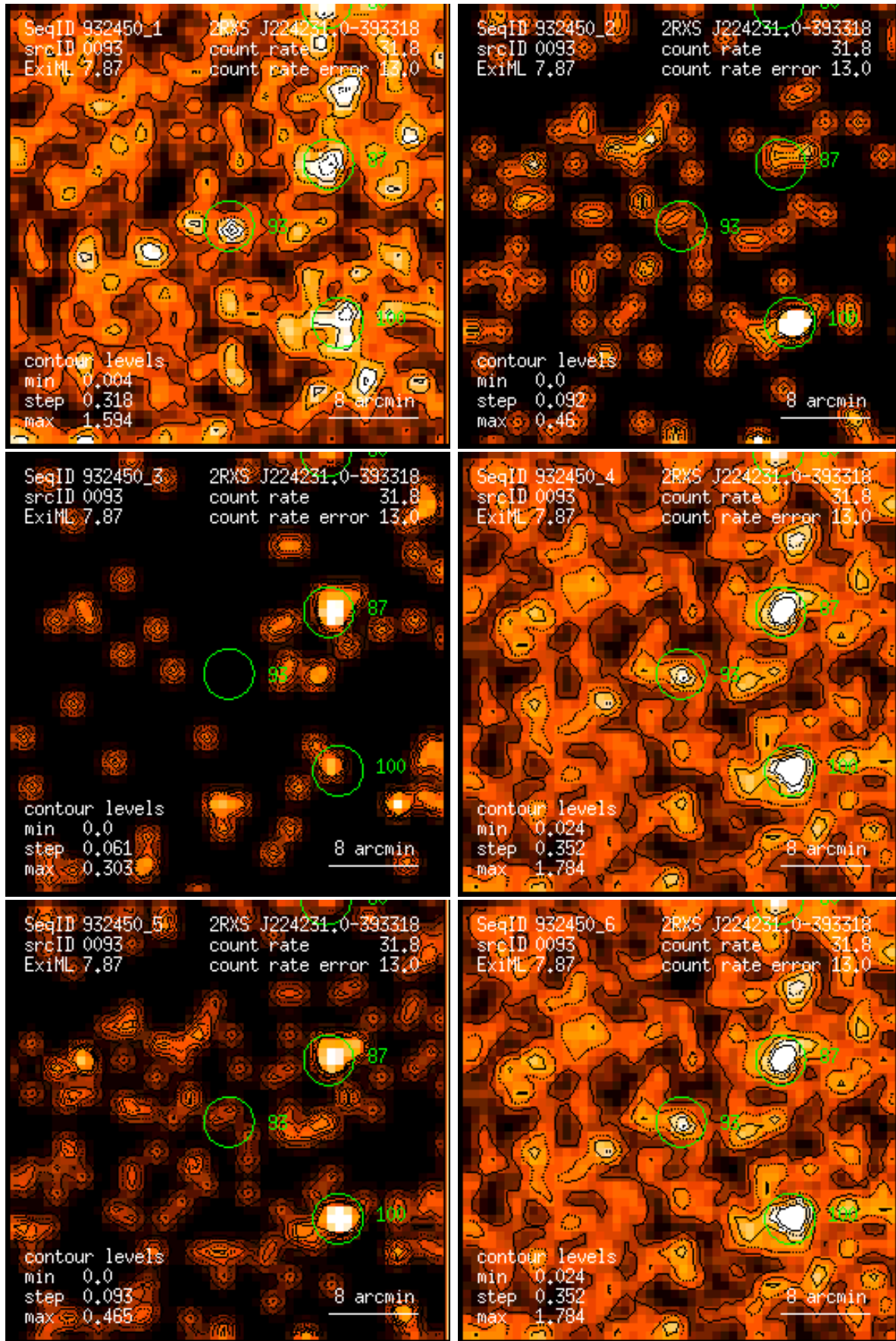
Figure 93: RASS 932450: detection 0093: band rate images, Gaussian filter: (1) PSPC channels 11 – 41, (2) 52 – 90, (3) 91 – 201, (4) 11 – 235, (5) 52 – 201, (6) 11 – 201. Broad band rates in counts/ks. Band rate contour levels in counts/ks/arcmin 2 .
