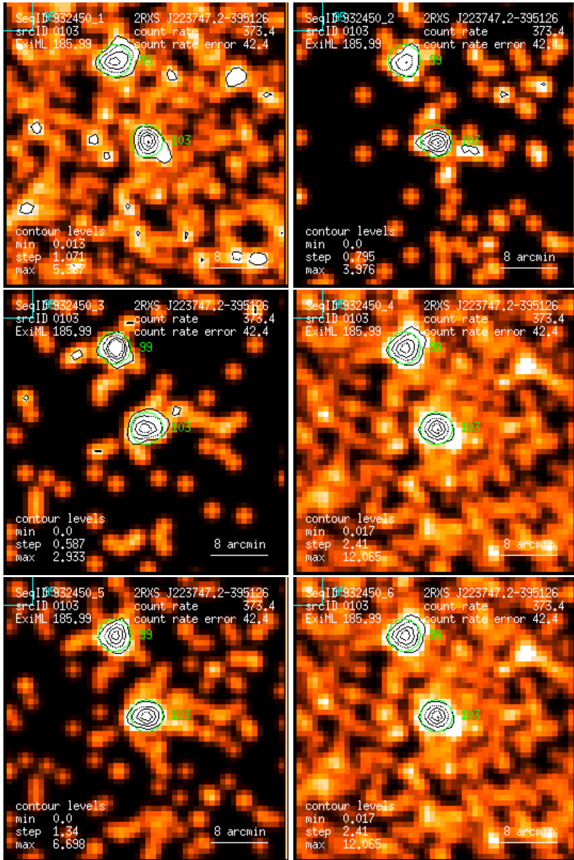
Figure 103: RASS 932450: detection 0103: band rate images, Gaussian filter: (1) PSPC channels 11 – 41, (2) 52 – 90, (3) 91 – 201, (4) 11 – 235, (5) 52 – 201, (6) 11 – 201. Broad band rates in counts/ks. Band rate contour levels in counts/ks/arcmin 2 .
