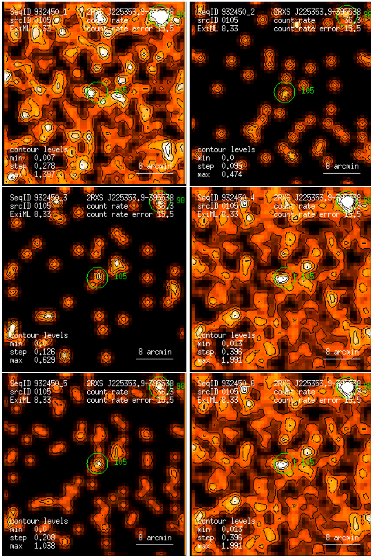
Figure 105: RASS 932450: detection 0105: band rate images, Gaussian filter: (1) PSPC channels 11 – 41, (2) 52 – 90, (3) 91 – 201, (4) 11 – 235, (5) 52 – 201, (6) 11 – 201. Broad band rates in counts/ks. Band rate contour levels in counts/ks/arcmin 2 .
