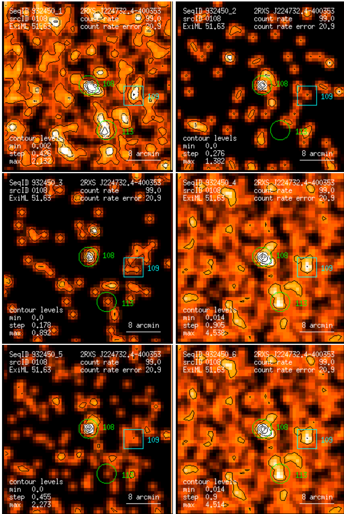
Figure 108: RASS 932450: detection 0108: band rate images, Gaussian filter: (1) PSPC channels 11 – 41, (2) 52 – 90, (3) 91 – 201, (4) 11 – 235, (5) 52 – 201, (6) 11 – 201. Broad band rates in counts/ks. Band rate contour levels in counts/ks/arcmin 2 .
