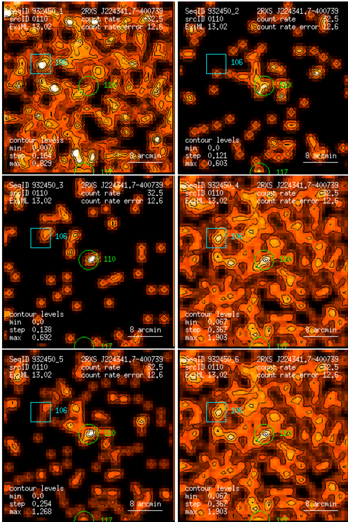
Figure 110: RASS 932450: detection 0110: band rate images, Gaussian filter: (1) PSPC channels 11 – 41, (2) 52 – 90, (3) 91 – 201, (4) 11 – 235, (5) 52 – 201, (6) 11 – 201. Broad band rates in counts/ks. Band rate contour levels in counts/ks/arcmin 2 .
