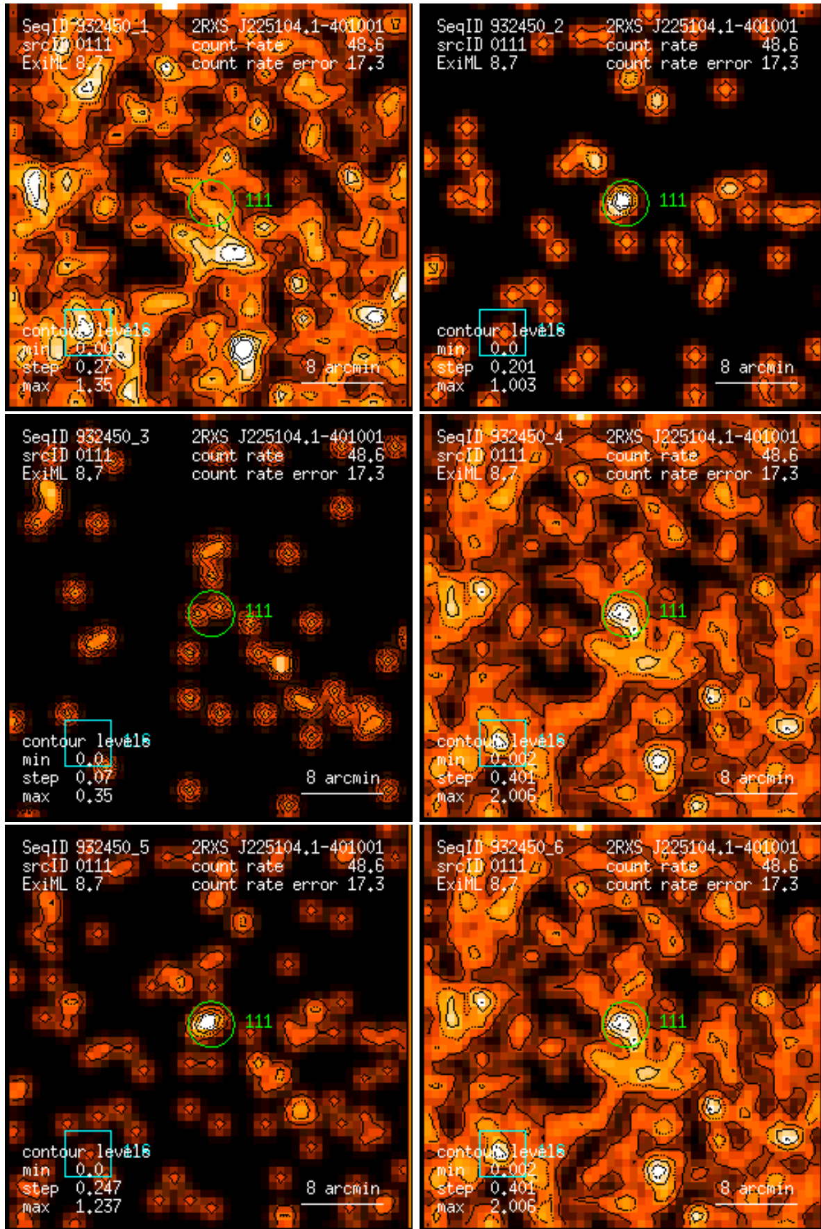
Figure 111: RASS 932450: detection 0111: band rate images, Gaussian filter: (1) PSPC channels 11 – 41, (2) 52 – 90, (3) 91 – 201, (4) 11 – 235, (5) 52 – 201, (6) 11 – 201. Broad band rates in counts/ks. Band rate contour levels in counts/ks/arcmin 2 .
