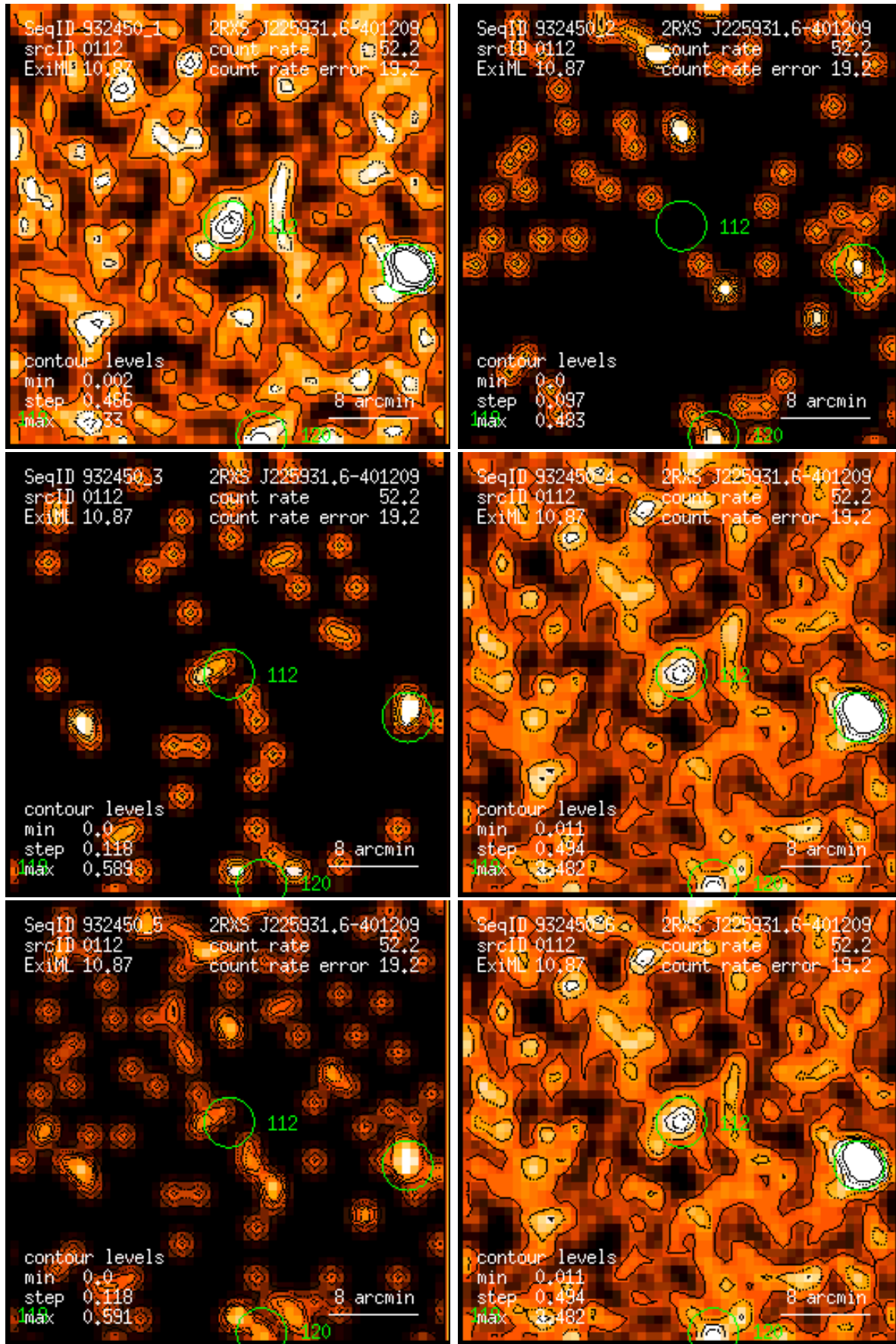
Figure 112: RASS 932450: detection 0112: band rate images, Gaussian filter: (1) PSPC channels 11 – 41, (2) 52 – 90, (3) 91 – 201, (4) 11 – 235, (5) 52 – 201, (6) 11 – 201. Broad band rates in counts/ks. Band rate contour levels in counts/ks/arcmin 2 .
