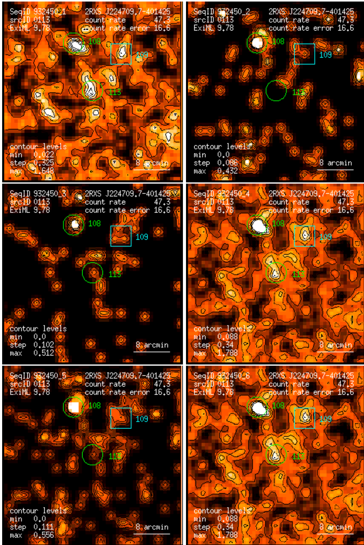
Figure 113: RASS 932450: detection 0113: band rate images, Gaussian filter: (1) PSPC channels 11 – 41, (2) 52 – 90, (3) 91 – 201, (4) 11 – 235, (5) 52 – 201, (6) 11 – 201. Broad band rates in counts/ks. Band rate contour levels in counts/ks/arcmin 2 .
