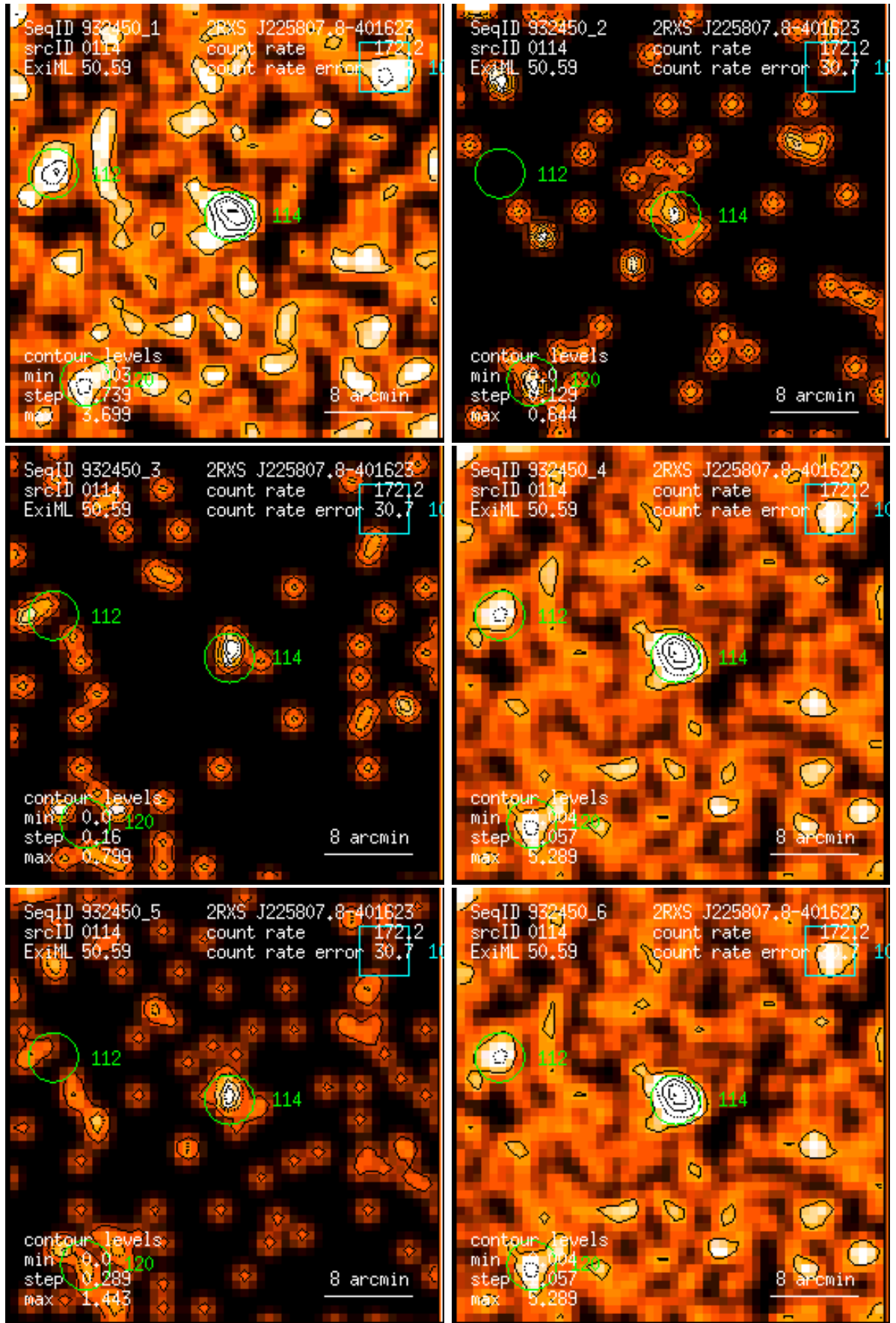
Figure 114: RASS 932450: detection 0114: band rate images, Gaussian filter: (1) PSPC channels 11 – 41, (2) 52 – 90, (3) 91 – 201, (4) 11 – 235, (5) 52 – 201, (6) 11 – 201. Broad band rates in counts/ks. Band rate contour levels in counts/ks/arcmin 2 .
