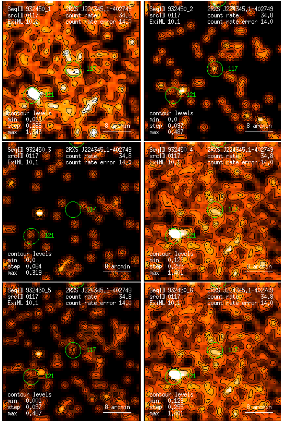
Figure 117: RASS 932450: detection 0117: band rate images, Gaussian filter: (1) PSPC channels 11 – 41, (2) 52 – 90, (3) 91 – 201, (4) 11 – 235, (5) 52 – 201, (6) 11 – 201. Broad band rates in counts/ks. Band rate contour levels in counts/ks/arcmin 2 .
