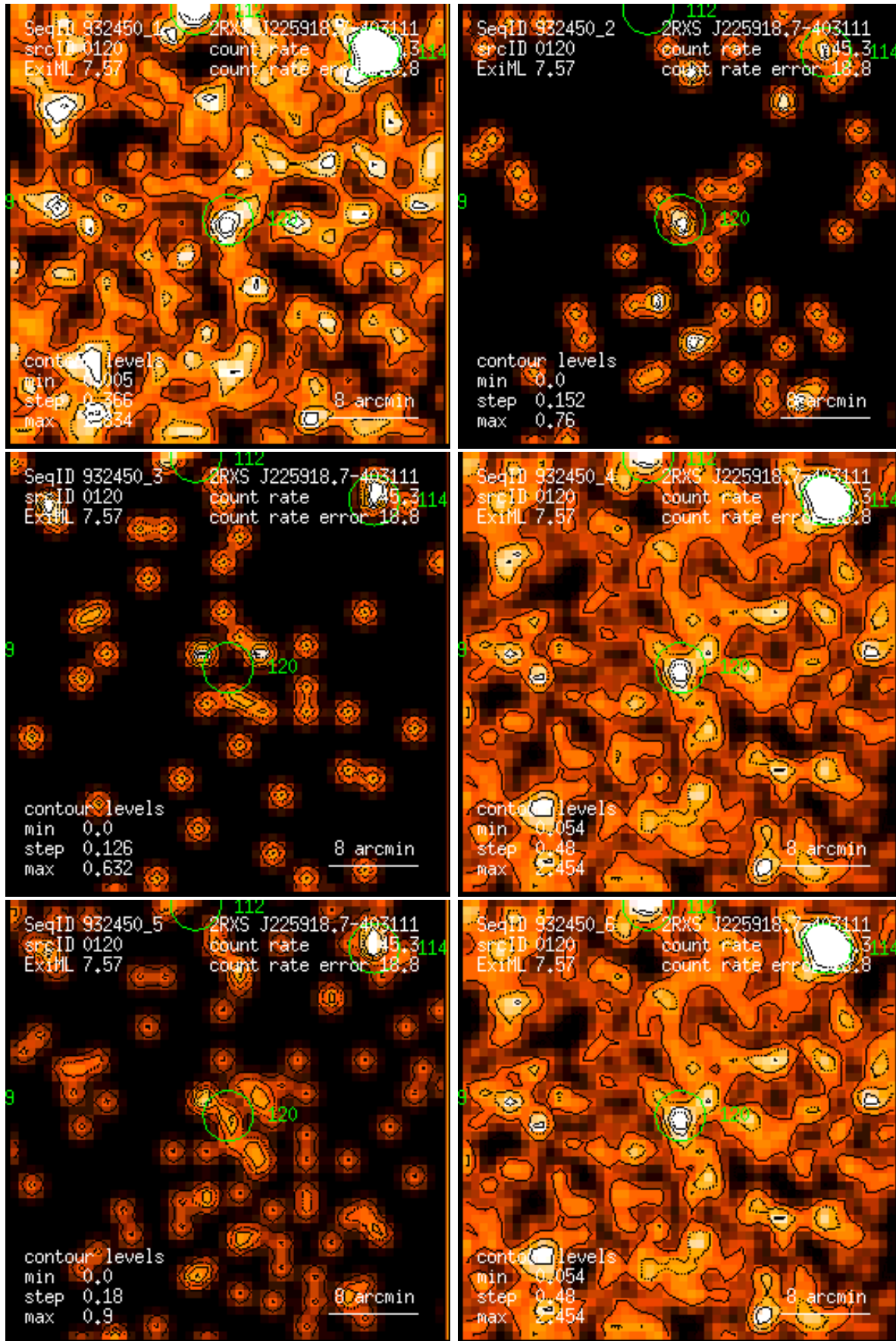
Figure 120: RASS 932450: detection 0120: band rate images, Gaussian filter: (1) PSPC channels 11 – 41, (2) 52 – 90, (3) 91 – 201, (4) 11 – 235, (5) 52 – 201, (6) 11 – 201. Broad band rates in counts/ks. Band rate contour levels in counts/ks/arcmin 2 .
