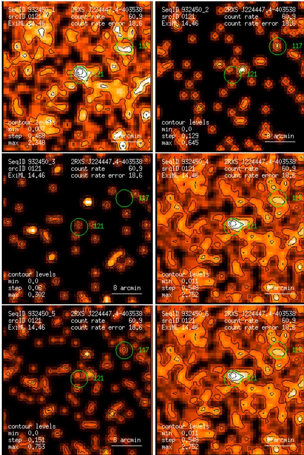
Figure 121: RASS 932450: detection 0121: band rate images, Gaussian filter: (1) PSPC channels 11 – 41, (2) 52 – 90, (3) 91 – 201, (4) 11 – 235, (5) 52 – 201, (6) 11 – 201. Broad band rates in counts/ks. Band rate contour levels in counts/ks/arcmin 2 .
