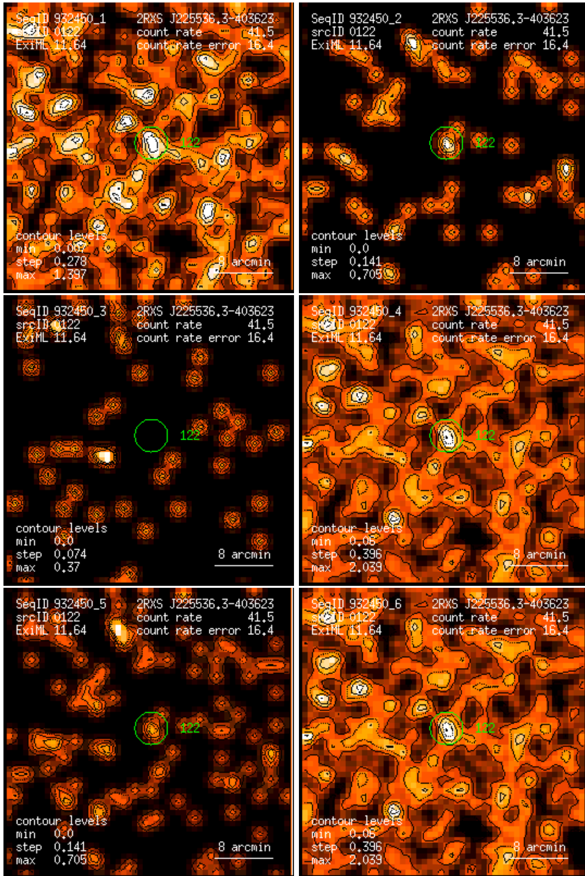
Figure 122: RASS 932450: detection 0122: band rate images, Gaussian filter: (1) PSPC channels 11 – 41, (2) 52 – 90, (3) 91 – 201, (4) 11 – 235, (5) 52 – 201, (6) 11 – 201. Broad band rates in counts/ks. Band rate contour levels in counts/ks/arcmin 2 .
