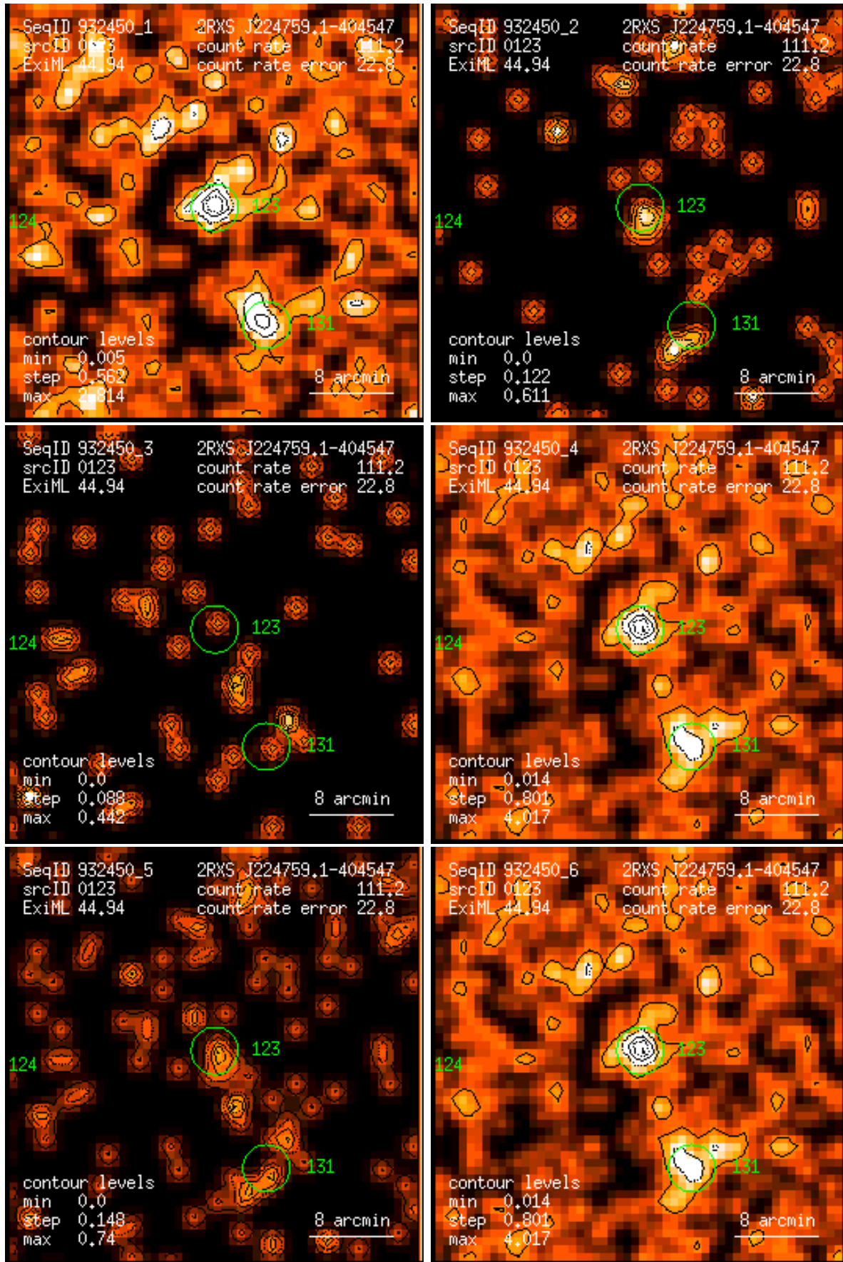
Figure 123: RASS 932450: detection 0123: band rate images, Gaussian filter: (1) PSPC channels 11 – 41, (2) 52 – 90, (3) 91 – 201, (4) 11 – 235, (5) 52 – 201, (6) 11 – 201. Broad band rates in counts/ks. Band rate contour levels in counts/ks/arcmin 2 .
