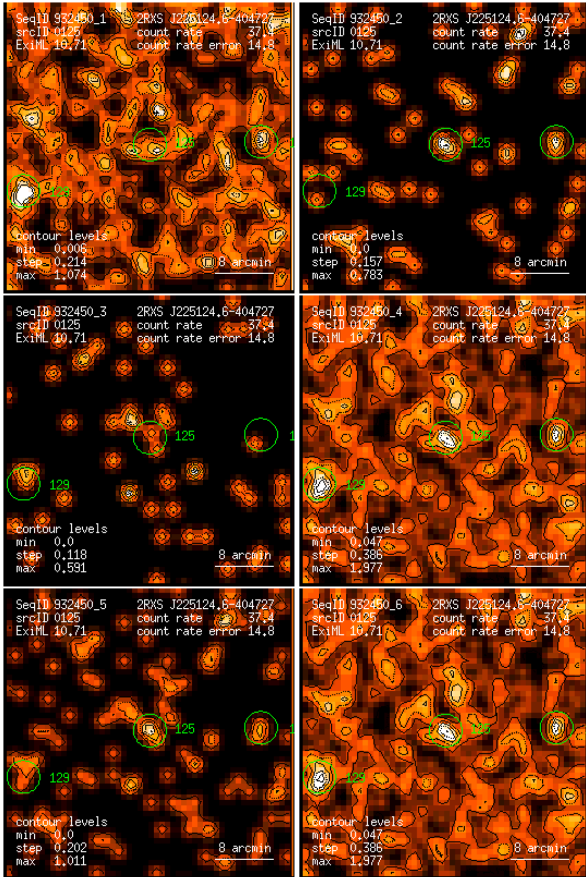
Figure 125: RASS 932450: detection 0125: band rate images, Gaussian filter: (1) PSPC channels 11 – 41, (2) 52 – 90, (3) 91 – 201, (4) 11 – 235, (5) 52 – 201, (6) 11 – 201. Broad band rates in counts/ks. Band rate contour levels in counts/ks/arcmin 2 .
