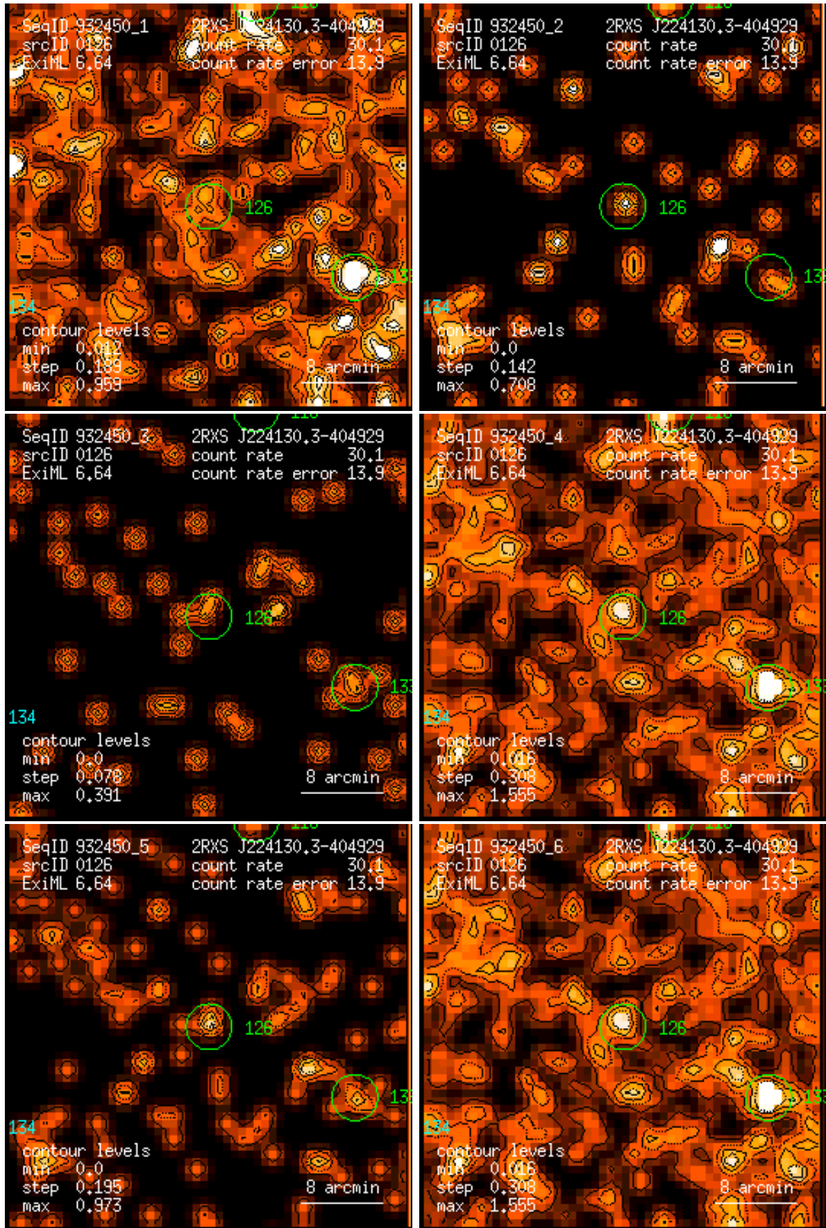
Figure 126: RASS 932450: detection 0126: band rate images, Gaussian filter: (1) PSPC channels 11 – 41, (2) 52 – 90, (3) 91 – 201, (4) 11 – 235, (5) 52 – 201, (6) 11 – 201. Broad band rates in counts/ks. Band rate contour levels in counts/ks/arcmin 2 .
