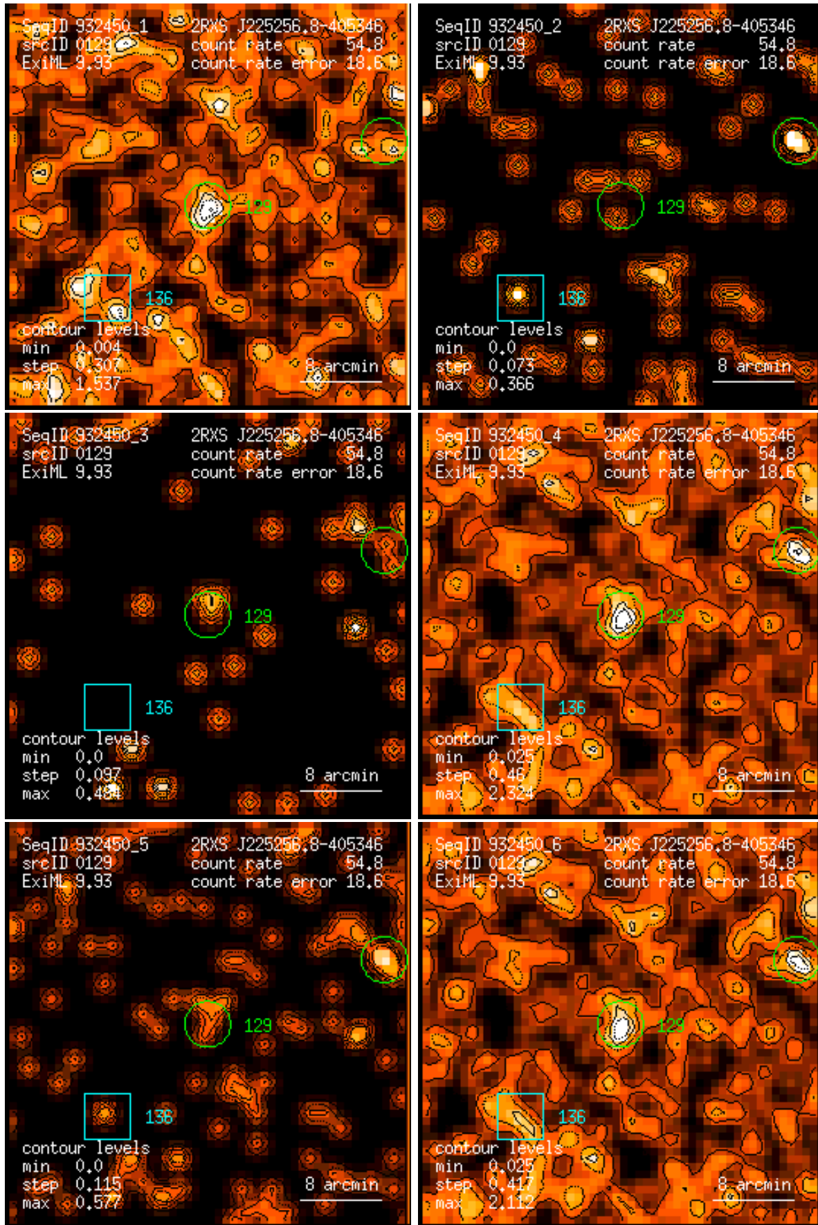
Figure 129: RASS 932450: detection 0129: band rate images, Gaussian filter: (1) PSPC channels 11 – 41, (2) 52 – 90, (3) 91 – 201, (4) 11 – 235, (5) 52 – 201, (6) 11 – 201. Broad band rates in counts/ks. Band rate contour levels in counts/ks/arcmin 2 .
