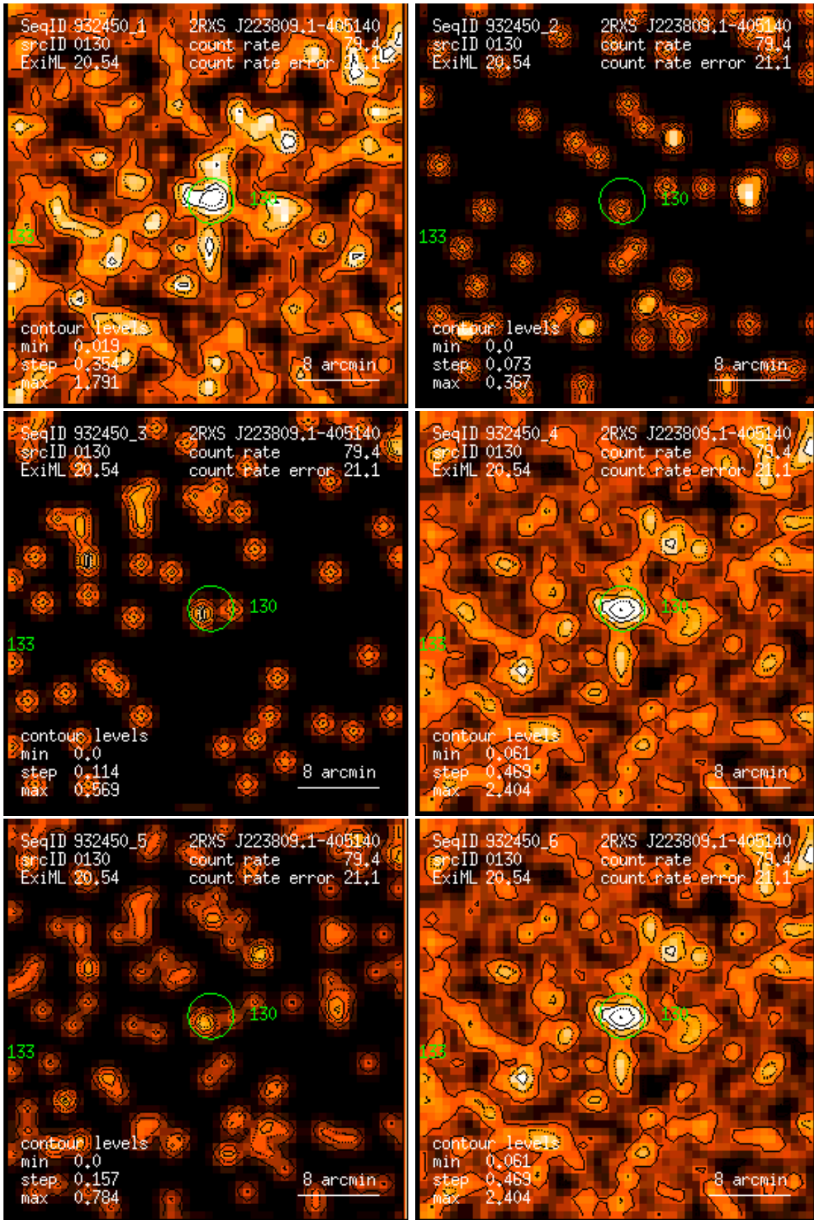
Figure 130: RASS 932450: detection 0130: band rate images, Gaussian filter: (1) PSPC channels 11 – 41, (2) 52 – 90, (3) 91 – 201, (4) 11 – 235, (5) 52 – 201, (6) 11 – 201. Broad band rates in counts/ks. Band rate contour levels in counts/ks/arcmin 2 .
