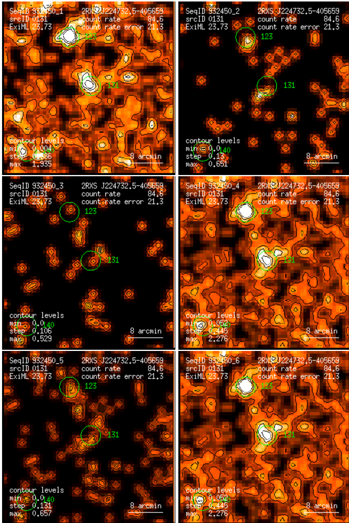
Figure 131: RASS 932450: detection 0131: band rate images, Gaussian filter: (1) PSPC channels 11 – 41, (2) 52 – 90, (3) 91 – 201, (4) 11 – 235, (5) 52 – 201, (6) 11 – 201. Broad band rates in counts/ks. Band rate contour levels in counts/ks/arcmin 2 .
