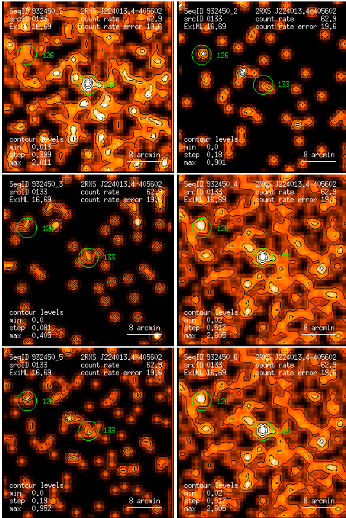
Figure 133: RASS 932450: detection 0133: band rate images, Gaussian filter: (1) PSPC channels 11 – 41, (2) 52 – 90, (3) 91 – 201, (4) 11 – 235, (5) 52 – 201, (6) 11 – 201. Broad band rates in counts/ks. Band rate contour levels in counts/ks/arcmin 2 .
