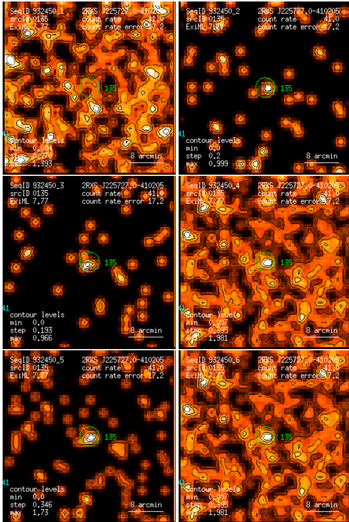
Figure 135: RASS 932450: detection 0135: band rate images, Gaussian filter: (1) PSPC channels 11 – 41, (2) 52 – 90, (3) 91 – 201, (4) 11 – 235, (5) 52 – 201, (6) 11 – 201. Broad band rates in counts/ks. Band rate contour levels in counts/ks/arcmin 2 .
