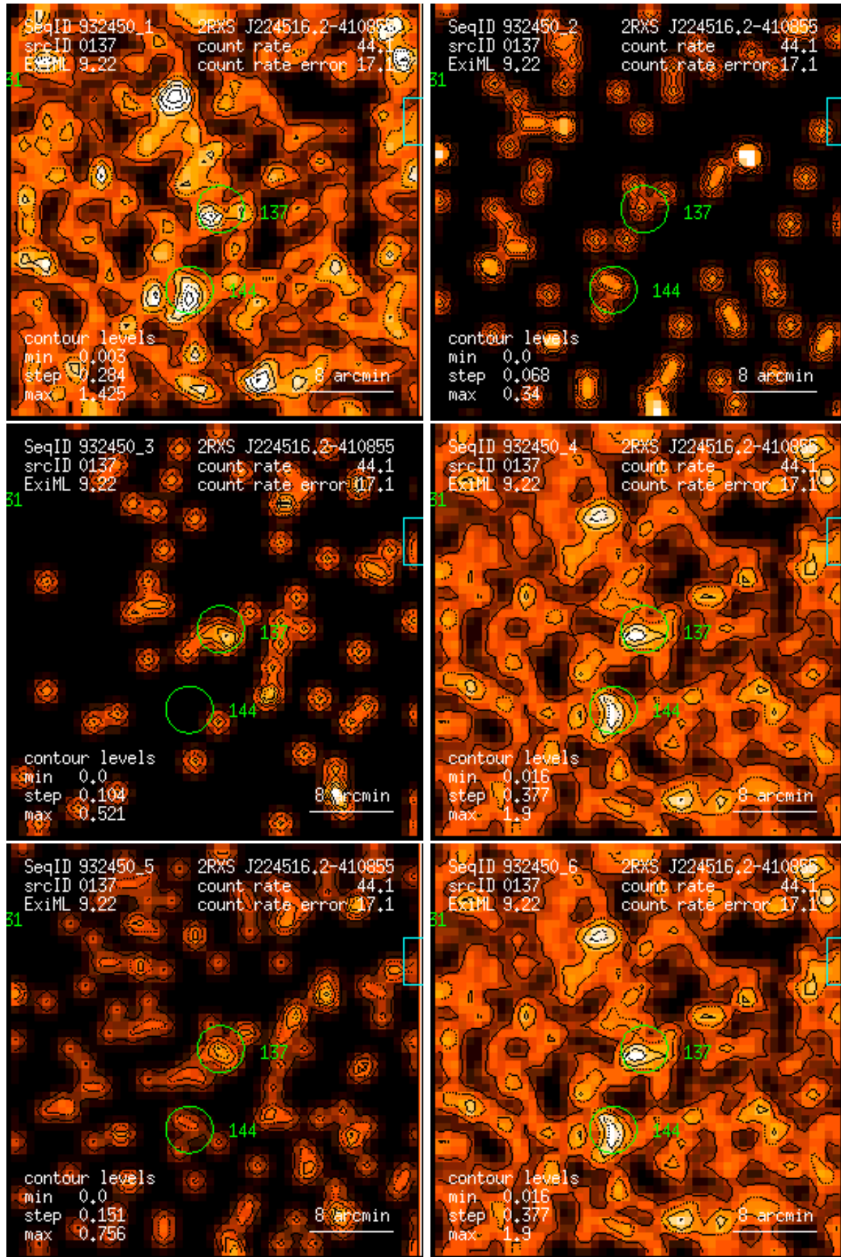
Figure 137: RASS 932450: detection 0137: band rate images, Gaussian filter: (1) PSPC channels 11 – 41, (2) 52 – 90, (3) 91 – 201, (4) 11 – 235, (5) 52 – 201, (6) 11 – 201. Broad band rates in counts/ks. Band rate contour levels in counts/ks/arcmin 2 .
