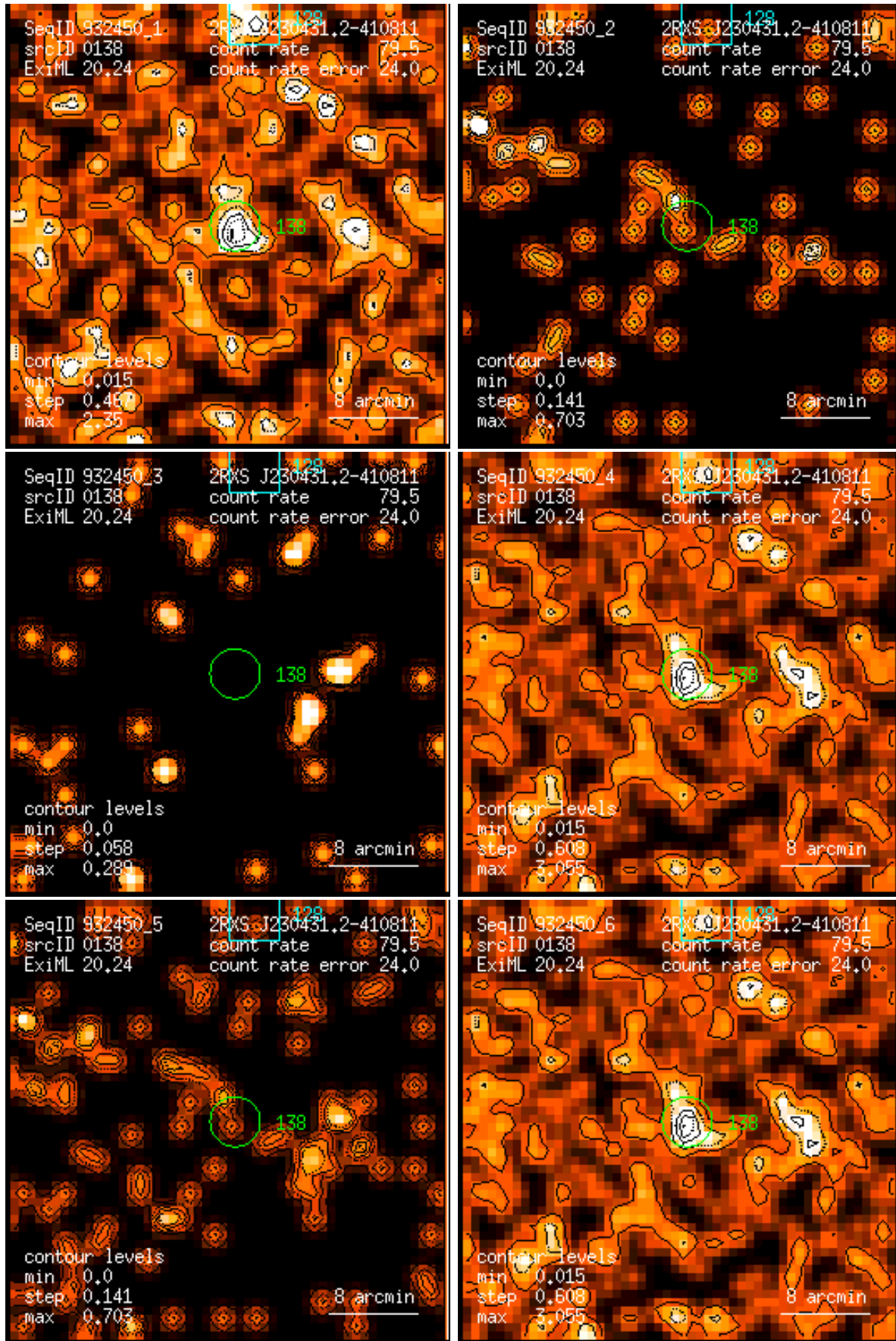
Figure 138: RASS 932450: detection 0138: band rate images, Gaussian filter: (1) PSPC channels 11 – 41, (2) 52 – 90, (3) 91 – 201, (4) 11 – 235, (5) 52 – 201, (6) 11 – 201. Broad band rates in counts/ks. Band rate contour levels in counts/ks/arcmin 2 .
