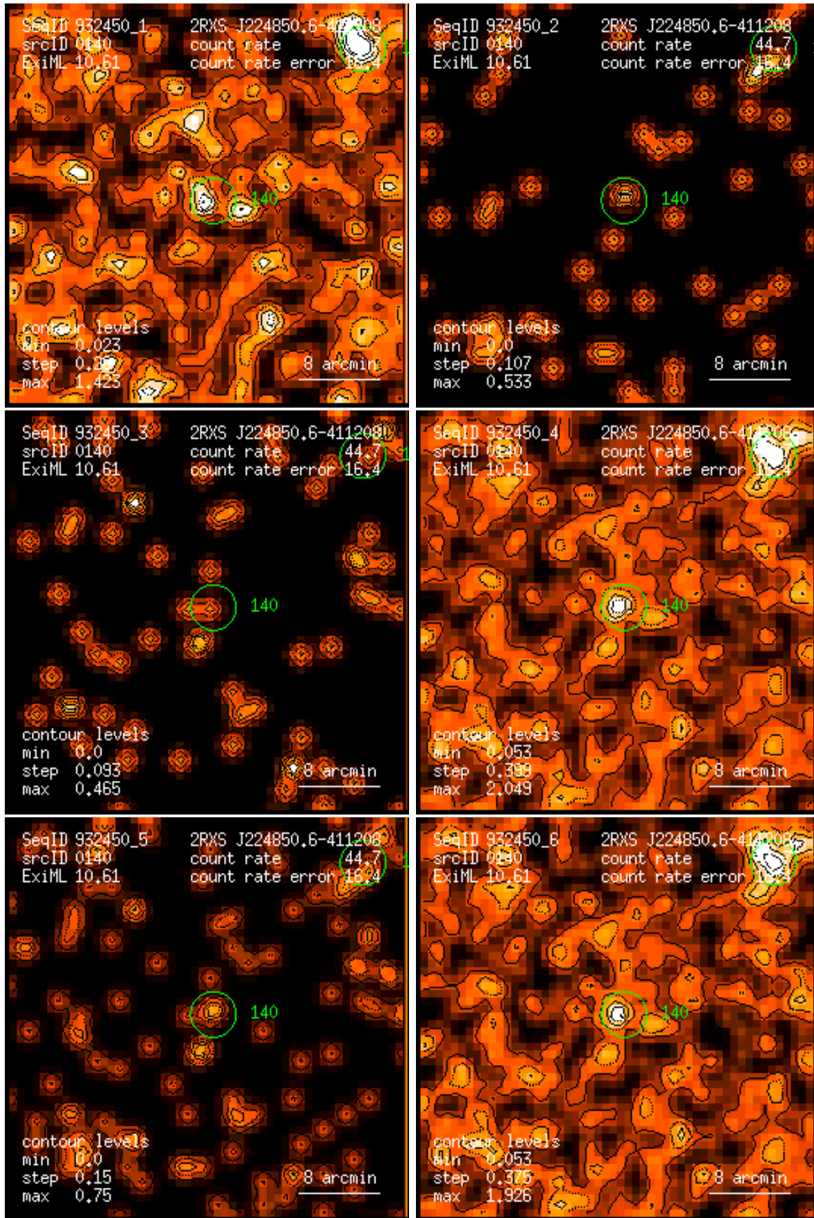
Figure 140: RASS 932450: detection 0140: band rate images, Gaussian filter: (1) PSPC channels 11 – 41, (2) 52 – 90, (3) 91 – 201, (4) 11 – 235, (5) 52 – 201, (6) 11 – 201. Broad band rates in counts/ks. Band rate contour levels in counts/ks/arcmin 2 .
