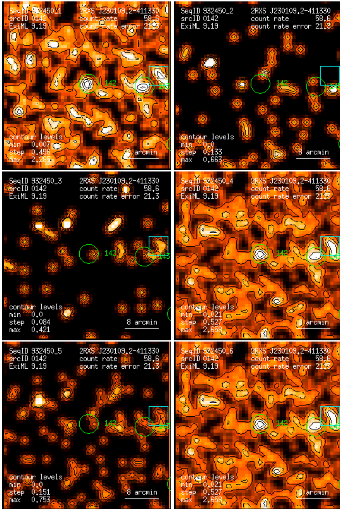
Figure 142: RASS 932450: detection 0142: band rate images, Gaussian filter: (1) PSPC channels 11 – 41, (2) 52 – 90, (3) 91 – 201, (4) 11 – 235, (5) 52 – 201, (6) 11 – 201. Broad band rates in counts/ks. Band rate contour levels in counts/ks/arcmin 2 .
