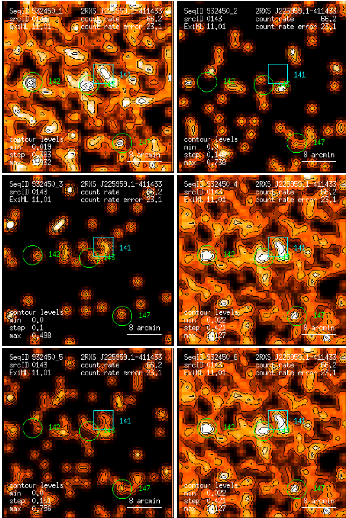
Figure 143: RASS 932450: detection 0143: band rate images, Gaussian filter: (1) PSPC channels 11 – 41, (2) 52 – 90, (3) 91 – 201, (4) 11 – 235, (5) 52 – 201, (6) 11 – 201. Broad band rates in counts/ks. Band rate contour levels in counts/ks/arcmin 2 .
