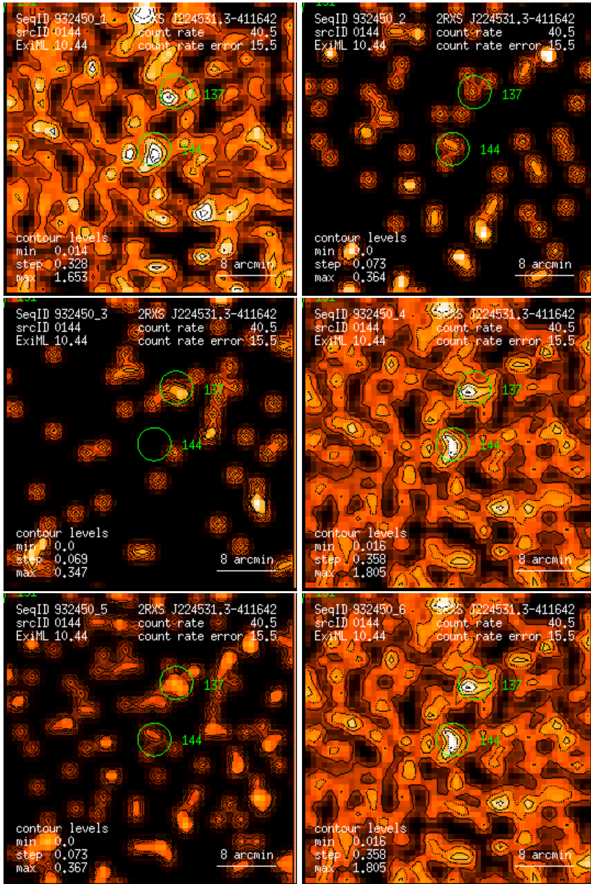
Figure 144: RASS 932450: detection 0144: band rate images, Gaussian filter: (1) PSPC channels 11 – 41, (2) 52 – 90, (3) 91 – 201, (4) 11 – 235, (5) 52 – 201, (6) 11 – 201. Broad band rates in counts/ks. Band rate contour levels in counts/ks/arcmin 2 .
