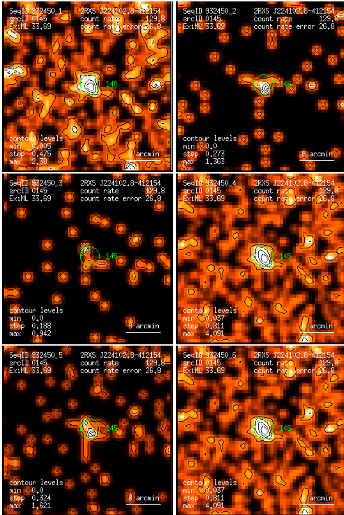
Figure 145: RASS 932450: detection 0145: band rate images, Gaussian filter: (1) PSPC channels 11 – 41, (2) 52 – 90, (3) 91 – 201, (4) 11 – 235, (5) 52 – 201, (6) 11 – 201. Broad band rates in counts/ks. Band rate contour levels in counts/ks/arcmin 2 .
