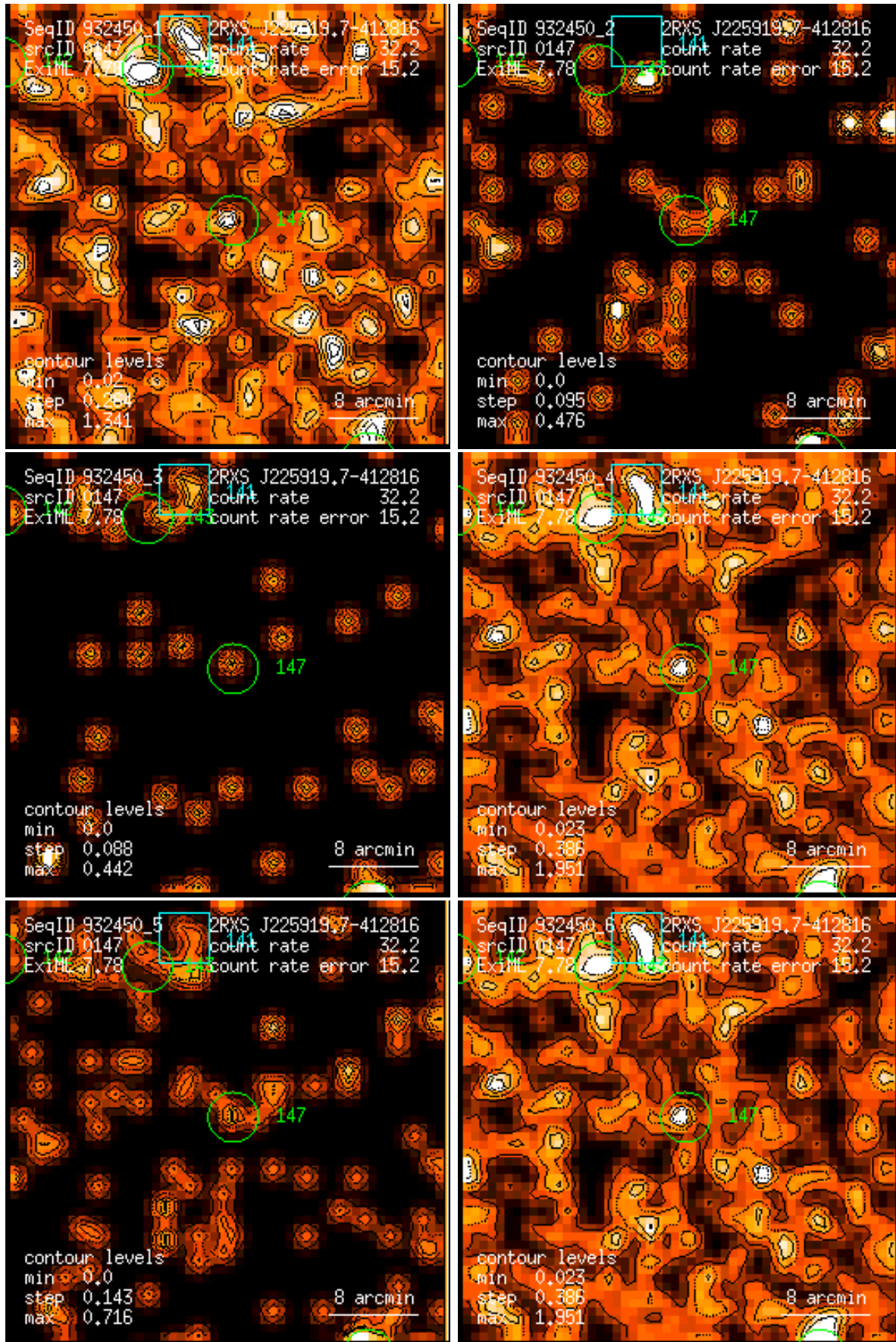
Figure 147: RASS 932450: detection 0147: band rate images, Gaussian filter: (1) PSPC channels 11 – 41, (2) 52 – 90, (3) 91 – 201, (4) 11 – 235, (5) 52 – 201, (6) 11 – 201. Broad band rates in counts/ks. Band rate contour levels in counts/ks/arcmin 2 .
