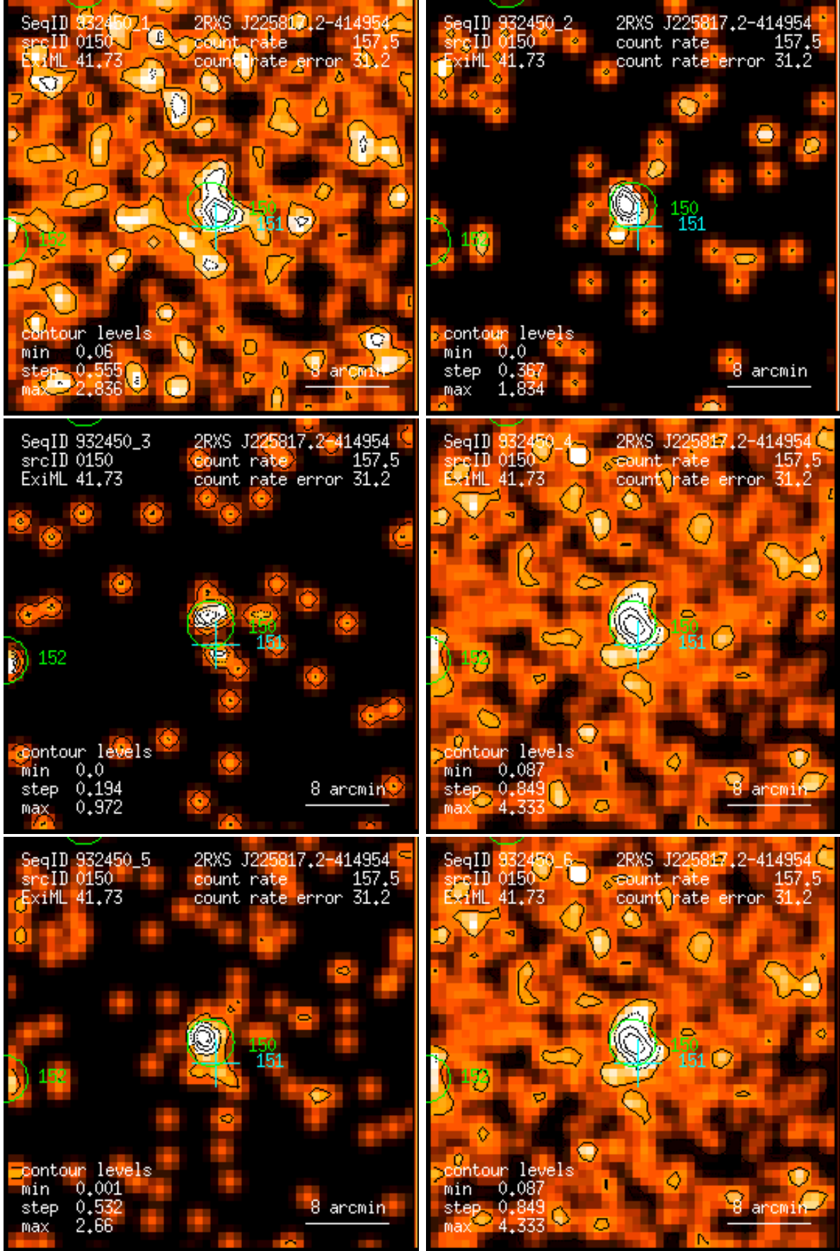
Figure 150: RASS 932450: detection 0150: band rate images, Gaussian filter: (1) PSPC channels 11 – 41, (2) 52 – 90, (3) 91 – 201, (4) 11 – 235, (5) 52 – 201, (6) 11 – 201. Broad band rates in counts/ks. Band rate contour levels in counts/ks/arcmin 2 .
