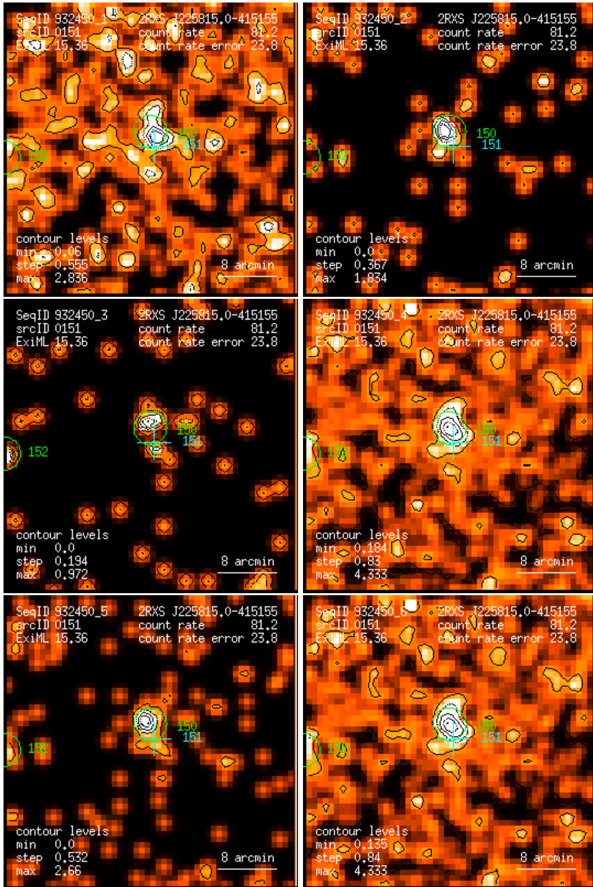
Figure 151: RASS 932450: detection 0151: band rate images, Gaussian filter: (1) PSPC channels 11 – 41, (2) 52 – 90, (3) 91 – 201, (4) 11 – 235, (5) 52 – 201, (6) 11 – 201. Broad band rates in counts/ks. Band rate contour levels in counts/ks/arcmin 2 .
