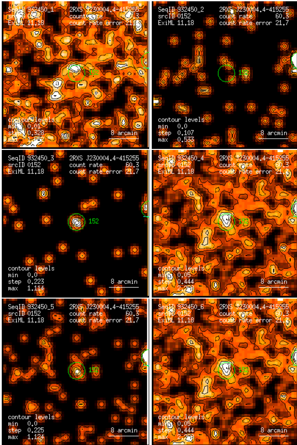
Figure 152: RASS 932450: detection 0152: band rate images, Gaussian filter: (1) PSPC channels 11 – 41, (2) 52 – 90, (3) 91 – 201, (4) 11 – 235, (5) 52 – 201, (6) 11 – 201. Broad band rates in counts/ks. Band rate contour levels in counts/ks/arcmin 2 .
