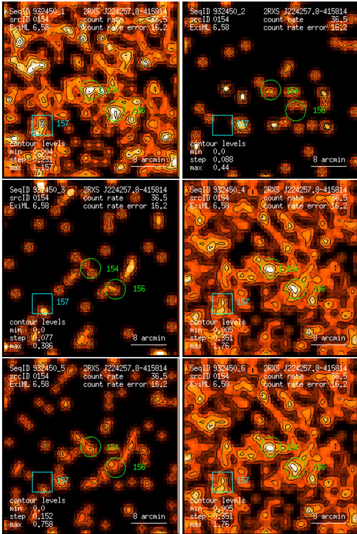
Figure 154: RASS 932450: detection 0154: band rate images, Gaussian filter: (1) PSPC channels 11 – 41, (2) 52 – 90, (3) 91 – 201, (4) 11 – 235, (5) 52 – 201, (6) 11 – 201. Broad band rates in counts/ks. Band rate contour levels in counts/ks/arcmin 2 .
