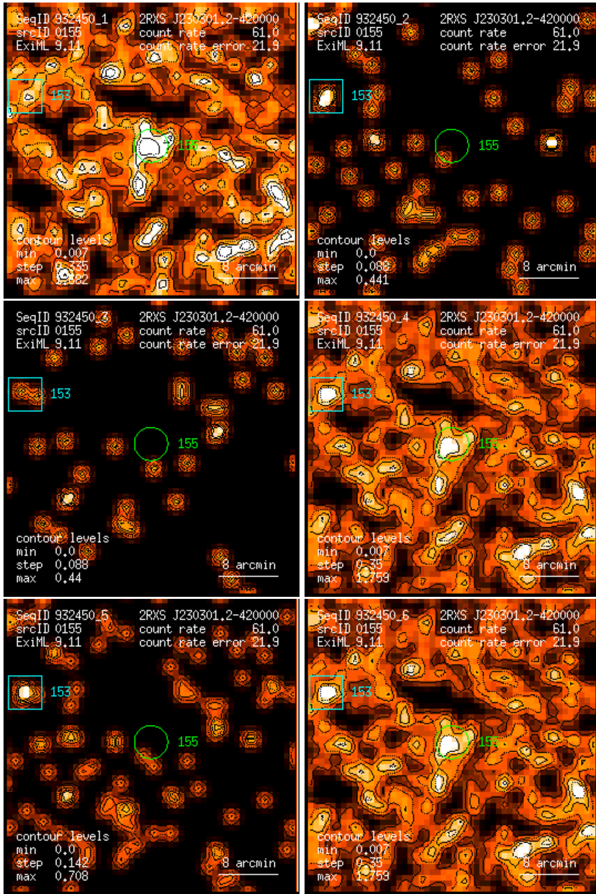
Figure 155: RASS 932450: detection 0155: band rate images, Gaussian filter: (1) PSPC channels 11 – 41, (2) 52 – 90, (3) 91 – 201, (4) 11 – 235, (5) 52 – 201, (6) 11 – 201. Broad band rates in counts/ks. Band rate contour levels in counts/ks/arcmin 2 .
