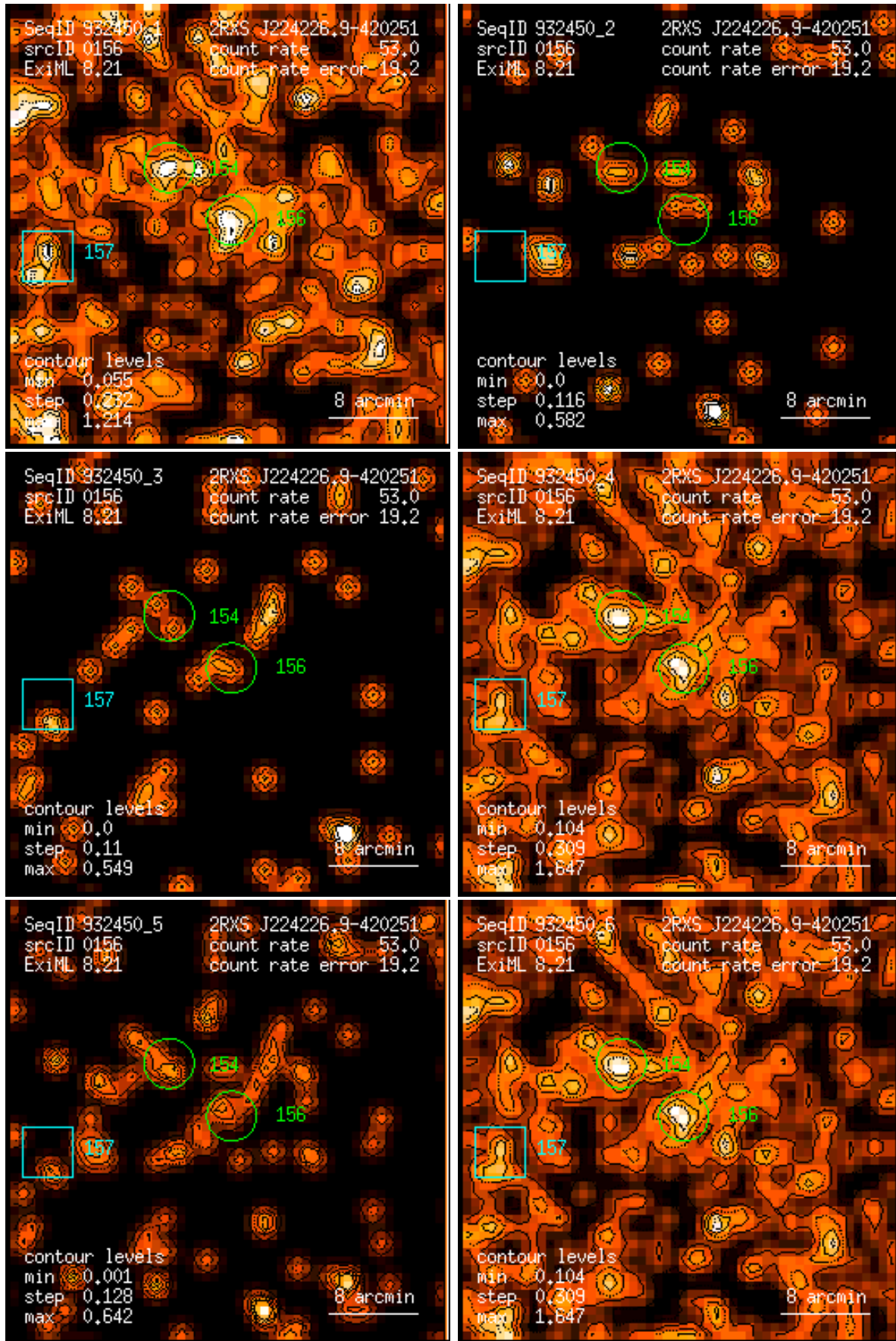
Figure 156: RASS 932450: detection 0156: band rate images, Gaussian filter: (1) PSPC channels 11 – 41, (2) 52 – 90, (3) 91 – 201, (4) 11 – 235, (5) 52 – 201, (6) 11 – 201. Broad band rates in counts/ks. Band rate contour levels in counts/ks/arcmin 2 .
