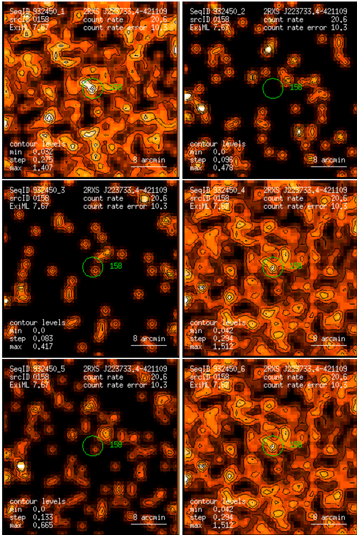
Figure 158: RASS 932450: detection 0158: band rate images, Gaussian filter: (1) PSPC channels 11 – 41, (2) 52 – 90, (3) 91 – 201, (4) 11 – 235, (5) 52 – 201, (6) 11 – 201. Broad band rates in counts/ks. Band rate contour levels in counts/ks/arcmin 2 .
