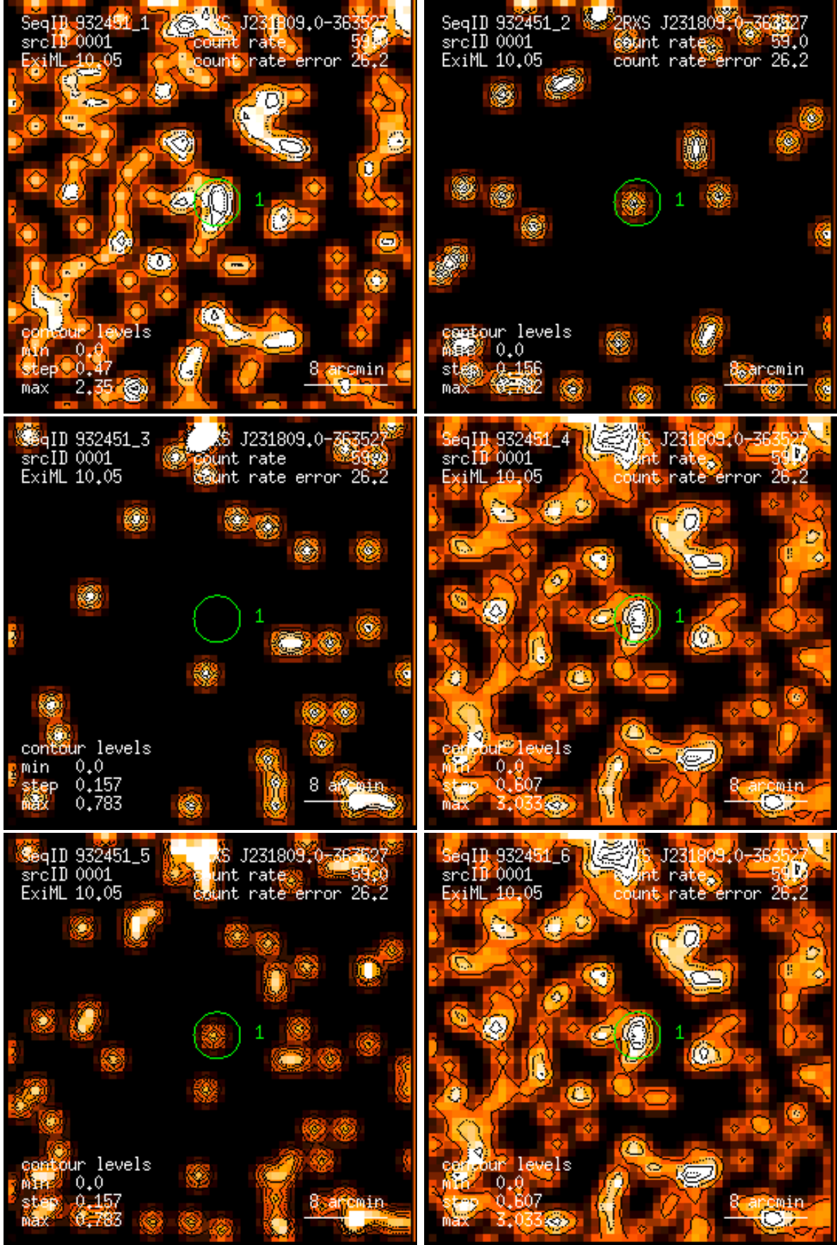
Figure 1: RASS 932451: detection 0001: band rate images, Gaussian filter: (1) PSPC channels 11 – 41, (2) 52 – 90, (3) 91 – 201, (4) 11 – 235, (5) 52 – 201, (6) 11 – 201. Broad band rates in counts/ks. Band rate contour levels in counts/ks/arcmin 2 .
