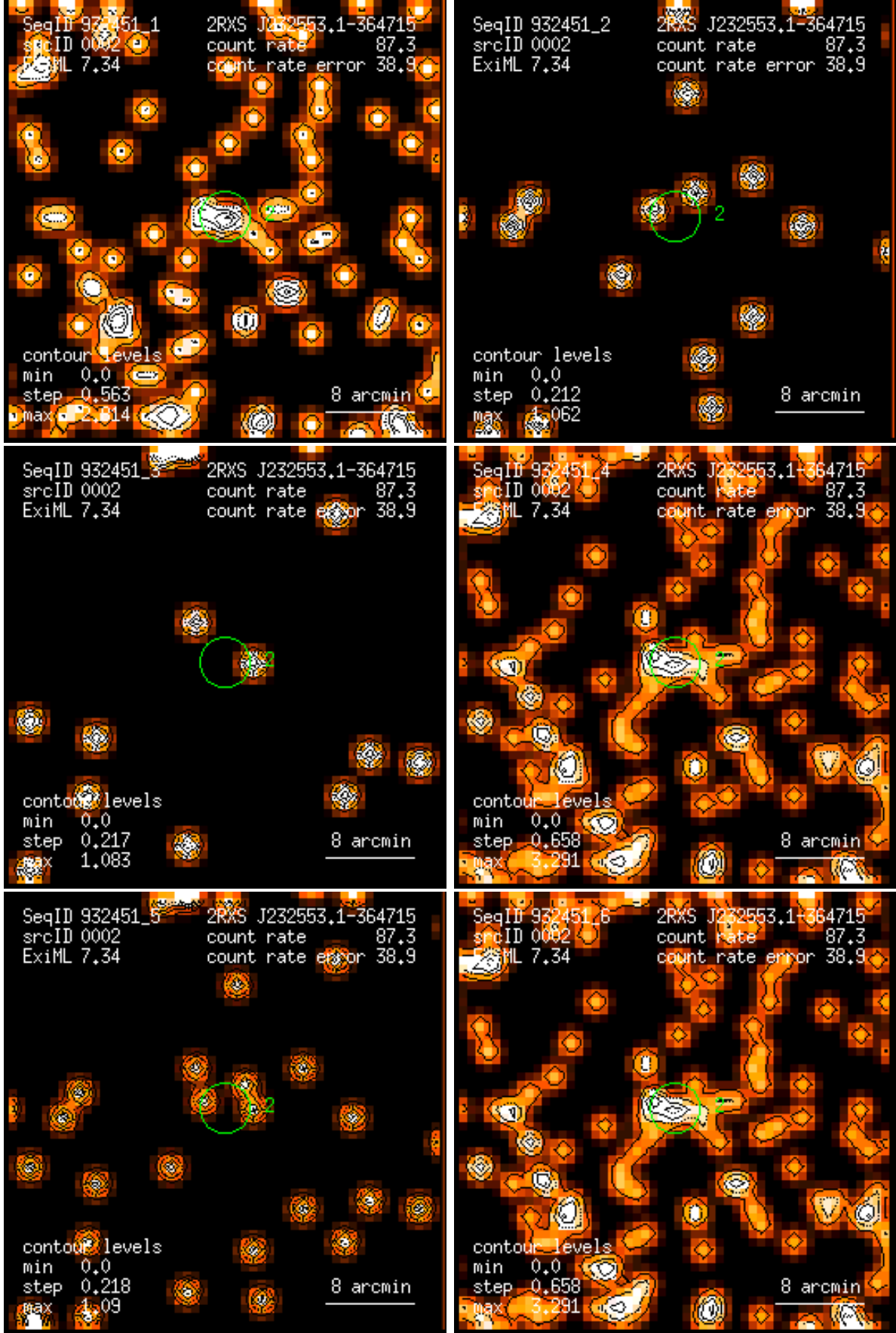
Figure 2: RASS 932451: detection 0002: band rate images, Gaussian filter: (1) PSPC channels 11 – 41, (2) 52 – 90, (3) 91 – 201, (4) 11 – 235, (5) 52 – 201, (6) 11 – 201. Broad band rates in counts/ks. Band rate contour levels in counts/ks/arcmin 2 .
