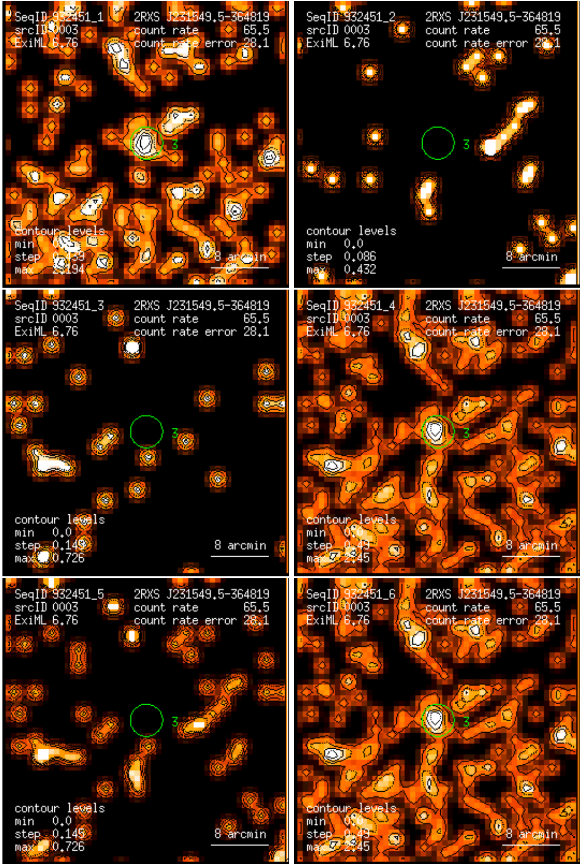
Figure 3: RASS 932451: detection 0003: band rate images, Gaussian filter: (1) PSPC channels 11 – 41, (2) 52 – 90, (3) 91 – 201, (4) 11 – 235, (5) 52 – 201, (6) 11 – 201. Broad band rates in counts/ks. Band rate contour levels in counts/ks/arcmin 2 .
