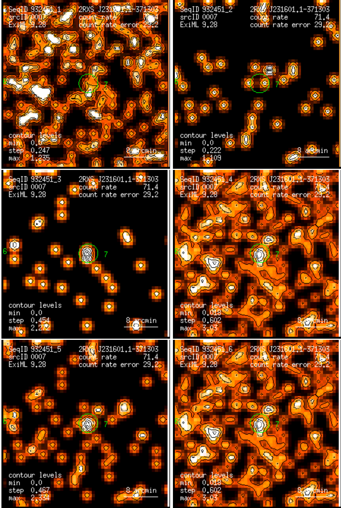
Figure 7: RASS 932451: detection 0007: band rate images, Gaussian filter: (1) PSPC channels 11 – 41, (2) 52 – 90, (3) 91 – 201, (4) 11 – 235, (5) 52 – 201, (6) 11 – 201. Broad band rates in counts/ks. Band rate contour levels in counts/ks/arcmin 2 .
