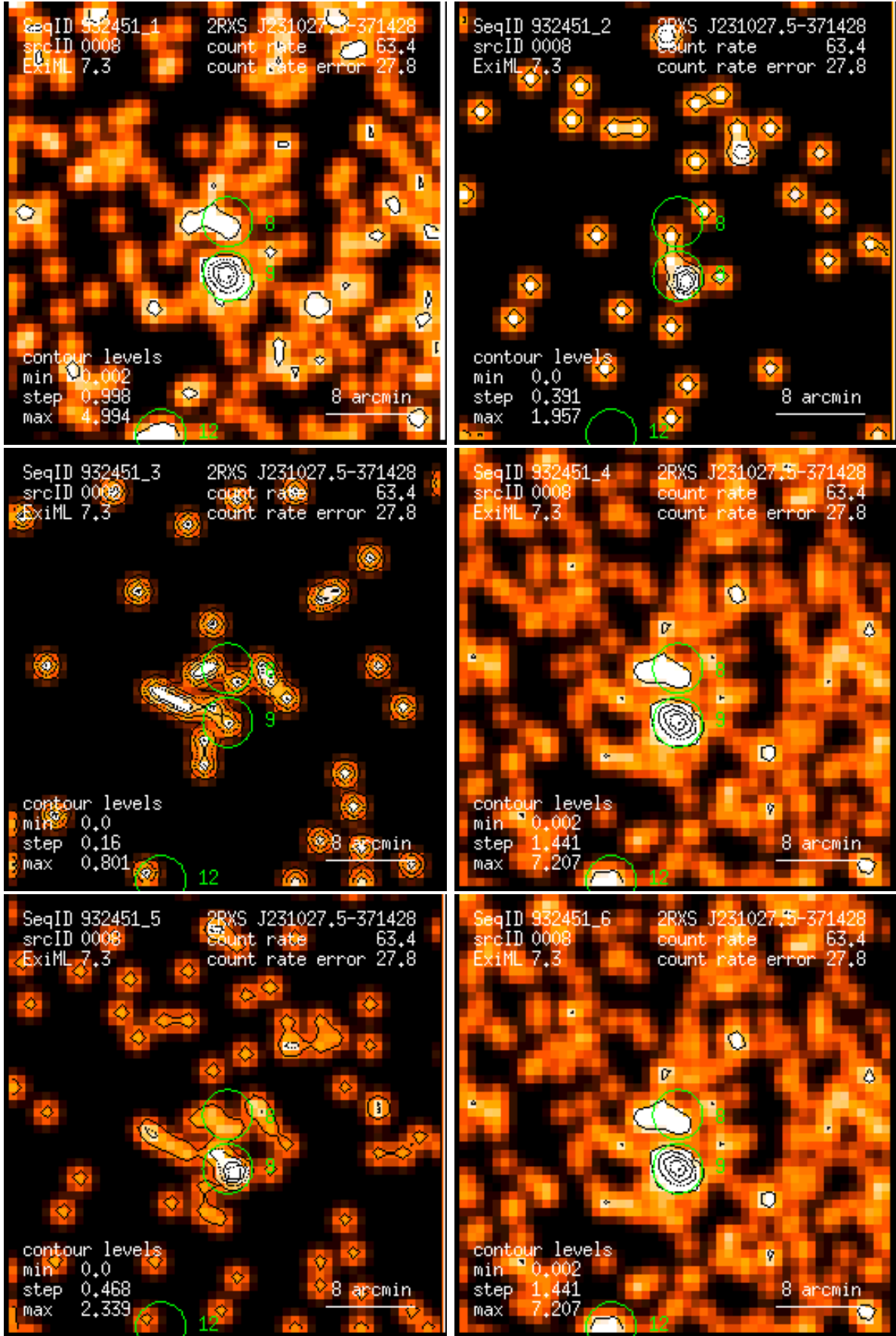
Figure 8: RASS 932451: detection 0008: band rate images, Gaussian filter: (1) PSPC channels 11 – 41, (2) 52 – 90, (3) 91 – 201, (4) 11 – 235, (5) 52 – 201, (6) 11 – 201. Broad band rates in counts/ks. Band rate contour levels in counts/ks/arcmin 2 .
